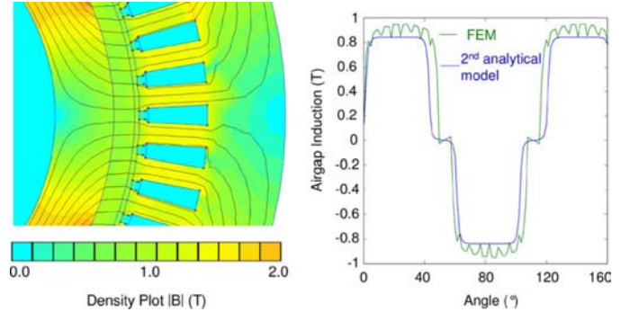
Fig. 9. Flux density in the PMSG airgap.
