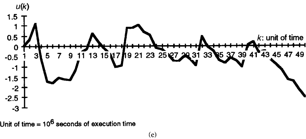
Figure 10.11 Trend tests for SS4. (a) Arithmetical mean of the times to failure. (b) Laplace factor of the times to failure. (c) Laplace factor of the failure intensity.
