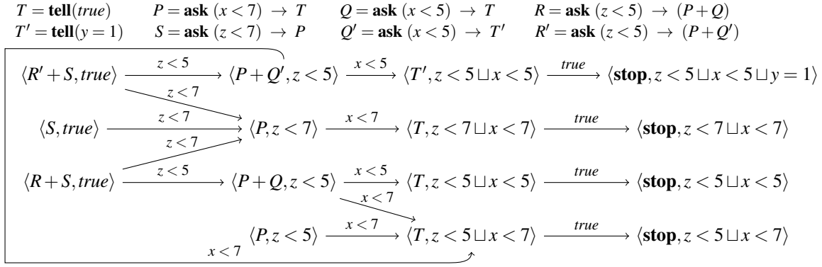
Figure 1: The LTS of the running example ( IS = \{\langle R' + S, true \rangle, \langle S, true \rangle, \langle R + S, true \rangle\} ).
