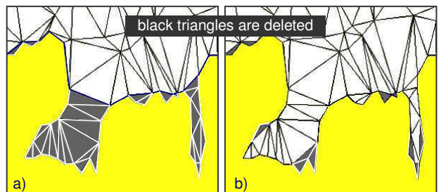
Figure 4: Deletion of potentially badly oriented triangles which preserves (b), or not (a), some significant details of the contour.
