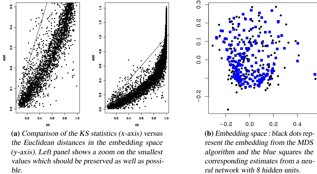
Figure 4: Embedding space computation with the Multidimensional scaling (MDS) algorithm applied to the Kolmogorov-Smirnov (KS) statistics as a measure of similarity on the synthetic data set B . The embedding space has dimension 2.
