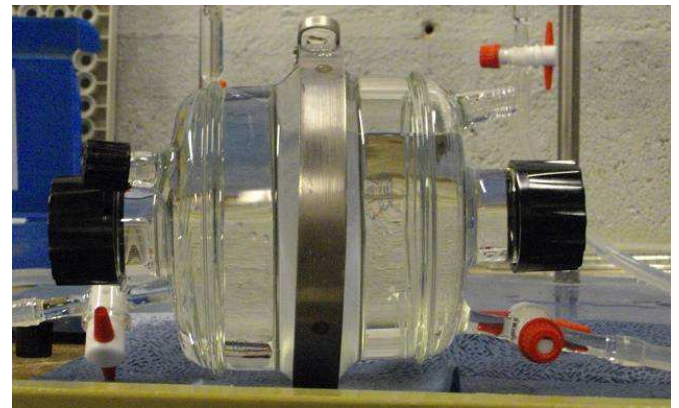
Figure 1 Diffusion cell with two identical parts separated by the geomembrane and linked with metallic bridge. This cell is identical to the control test cell
