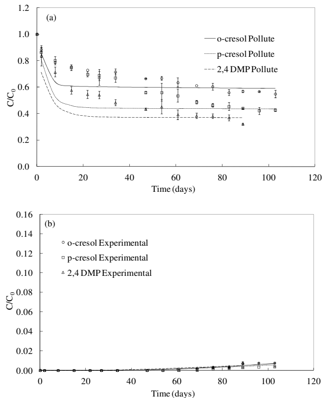
Figure 5 Evolution of the concentrations in (a) source and (b) receptor with time for methylphenols
