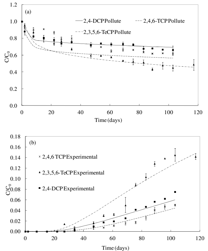
Figure 4 Evolution of the concentrations in (a) source and (b) receptor with time for chlorophenols
