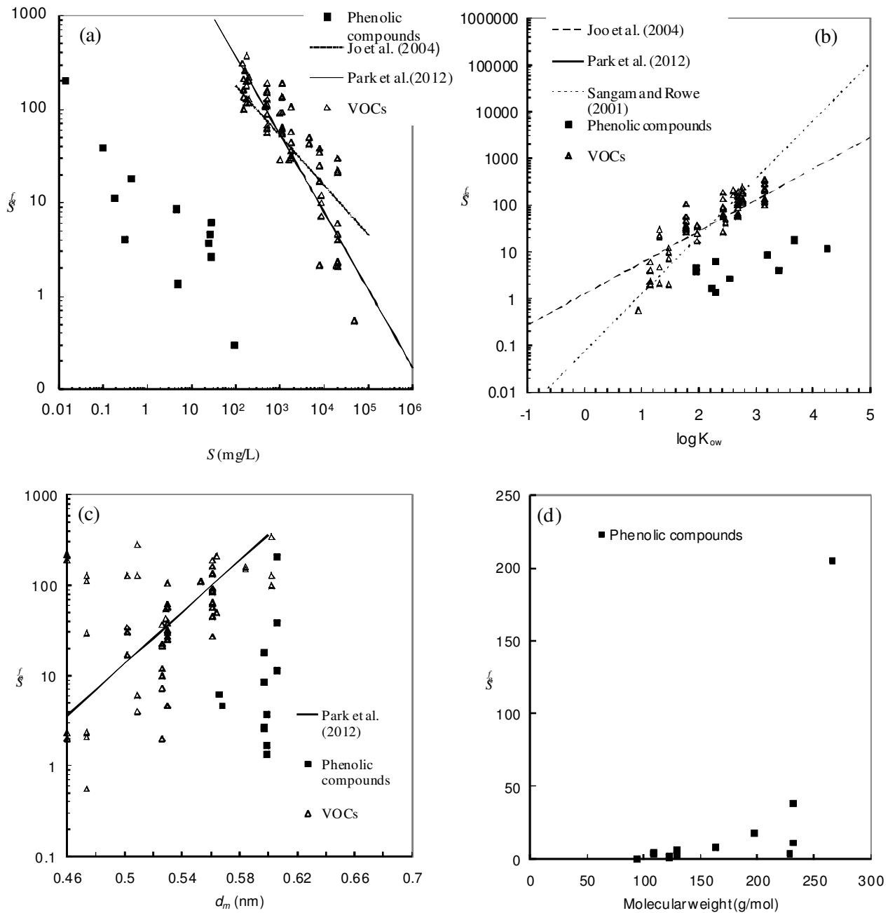
Figure 3 Relationship between partitioning coefficient, S_{gf} , and: (a) aqueous solubility, (b) octanol-water partitioning coefficient, K_{ow} , (c) molecular diameter, d_m , and (d) molecular weight for phenolic compounds and VOCs.
