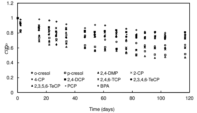
Figure 2 Observed normalized concentrations of the various phenolic compounds in control cells for diffusion tests.
