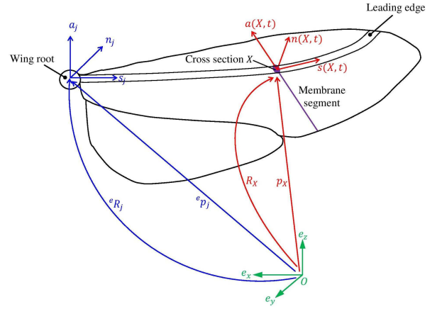
Fig. 3: Frames and parametrization of the soft wing.
