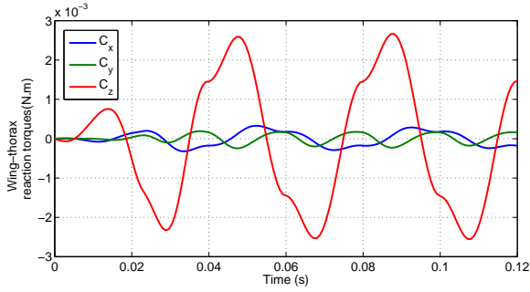
Fig. 8: Thorax-right wing reaction torques.
