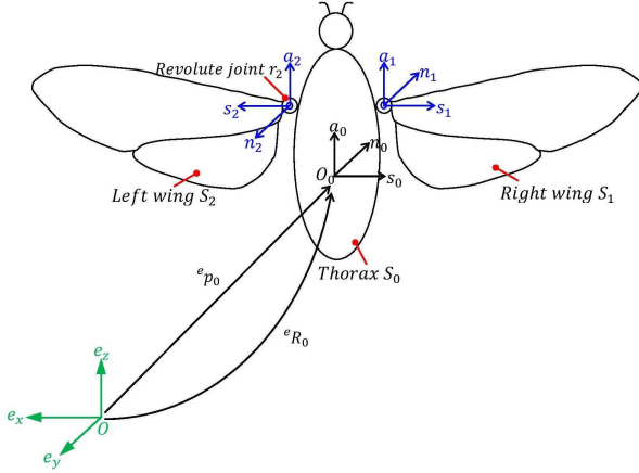
Fig. 1: Frames and parametrization of the insect-like MAV.
