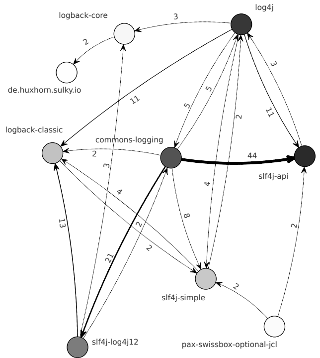
Fig. 5: Migration graphs for Logging libraries
