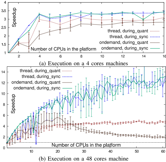
Fig. 9. Speedup Compared to SEQ for Different Implementation (average, min and max over 10 runs)
