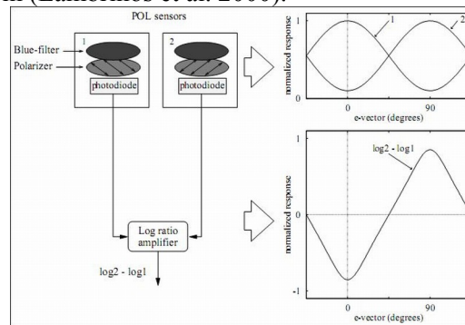
Figure 2: Diagrammatic description of POL OP unit. (Adapted from (Lambrinos et al., 2000; Chu et al., 2007))
