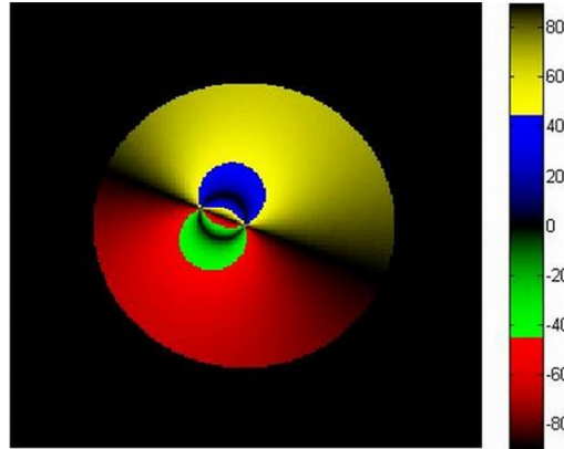
Figure 5: Simulation of the sky angle of polarization pattern in Le Creusot, France at 16:00 on 15-Mar-2011 using a pola-catadioptric sensor.
