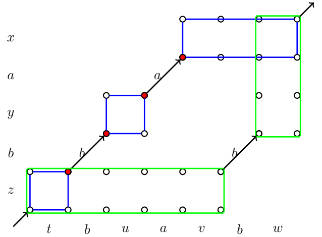
(b) An automaton which recognizes \sqcup(r, s) = (z \bullet t)b(u \bullet y)a(vbw \bullet x) \cup (tbuav \bullet z)b(w \bullet yax) . A rectangle holds for the shuffle of the factors on its sides
