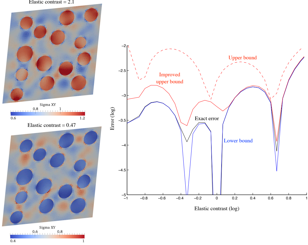
Figure 1: Error estimation of a POD-based reduced order model in the homogenisation of a particulate composite material.
