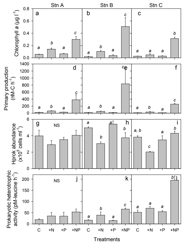
Fig. 4. Comparison of responses of chlorophyll- a ( \mu\text{g l}^{-1} ) (a, b, c), primary production ( \text{nM-C h}^{-1} ) (d, e, f), abundance of heterotrophic prokaryotes (Hprok) ( \text{cells ml}^{-1} ) (g, h, i), and prokaryotic heterotrophic activity ( \text{pM-leucine h}^{-1} ) (j, k, l) between the different treatments at the last day of the experiment. Values are shown as mean \pm SD. C, +N, +P, and +NP denote Control, \text{NH}_4 addition, \text{PO}_4 addition, \text{NH}_4+\text{PO}_4 addition, respectively. Columns labeled by different italic letters ( a or b ) are significantly different at P < 0.05 . NS denotes no significant effect of different nutrient treatments on the parameter measured. See Materials and methods for details.
