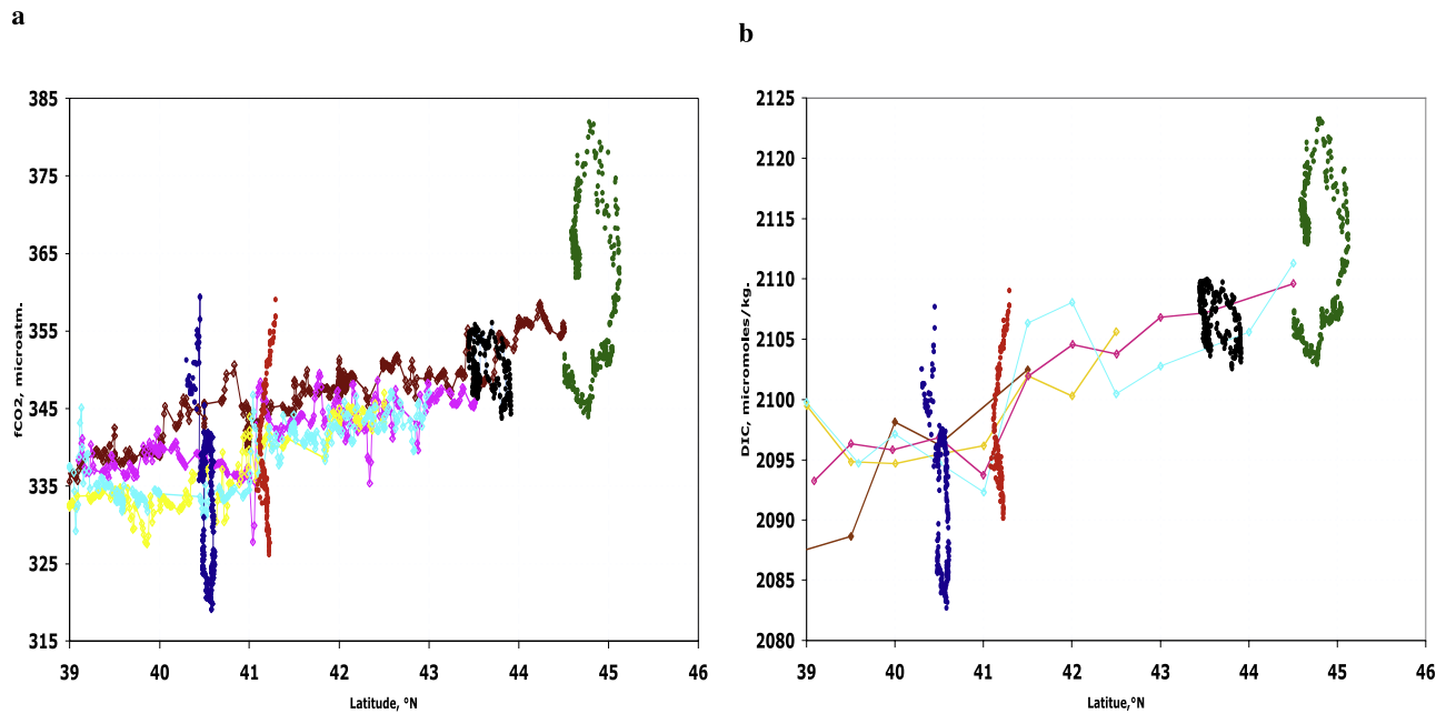
Figure 5. Latitudinal variations of (a) f\text{CO}_2 and (b) DIC measured along the north–south tracks of the R/V Atalante , shown as colored diamonds at 16.6^\circ\text{W} (brown), 18^\circ\text{W} (pink), 18.7^\circ\text{W} (cyan), and 19.3^\circ\text{W} (yellow) from 3 to 24 February and by the four buoys (dots with same color code as in Figure 1) after their deployment until 24 February.
