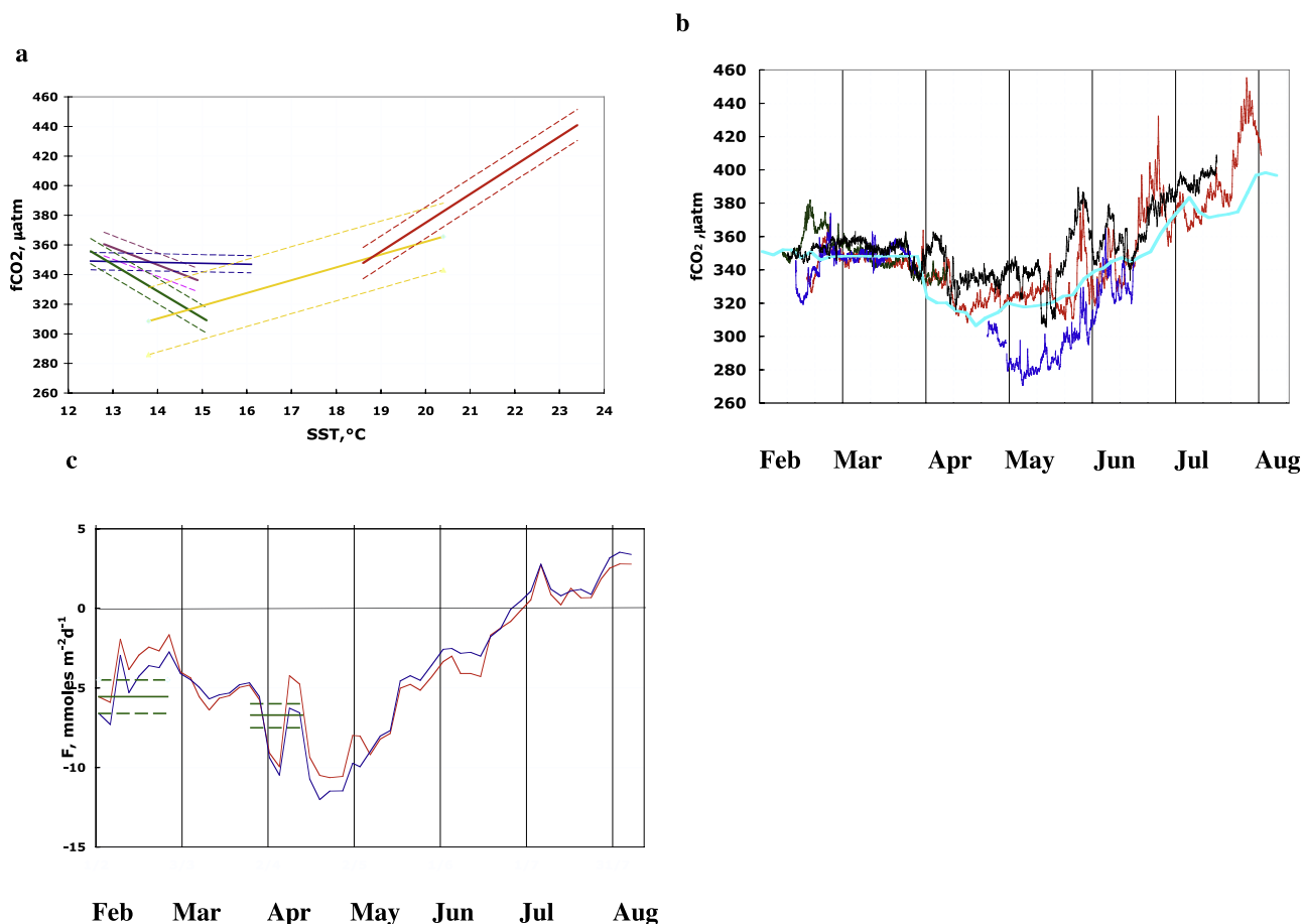
Figure 12. (a) fCO 2 /SST relationships for five periods: February (purple), March (blue), April (green), May–19 June (yellow), 20 June–1 August (red). The dotted lines indicate \pm 1 \sigma . (b) fCO 2 in \mu\text{atm} measured by the four buoys (same color code as in Figure 1b). The cyan line shows the interpolated values using satellite SST. (c) Air-sea CO 2 flux in \text{mmol m}^{-2} \text{day}^{-1} calculated over the POMME zone, 39^{\circ}\text{N}/45^{\circ}\text{N}-16^{\circ}\text{W}/21^{\circ}\text{W} (red), and on the enlarged zone, 36^{\circ}\text{N}/46^{\circ}\text{N}-12^{\circ}\text{W}/22^{\circ}\text{W} (blue). Each data point represents a 3–4 daytime interval. The green lines have been calculated by González-Dávila et al. using ship data. The full green line shows the mean value over the POMME zone. The dotted ones refer to the northern part, north of 42^{\circ}\text{N} , and the southern one, south of 42^{\circ}\text{N} . Negative values indicate that the ocean is a sink for atmospheric CO 2 .
