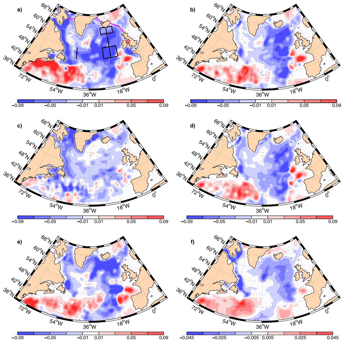
Figure 1. Mean annual salinity anomaly in year 5 in (a) experiment NAO in the upper 500 m, (b) experiment NAO in the 200–500 m layer; (c) experiment WIND-ARCT in the upper 500 m layer; (d) experiment WIND in the 200–500 m layer; (e) Mean annual salinity anomaly in year 7 in experiment NAO in the 200–500 m layer; (f) First EOF of the mean annual salinity in the 200–500 m layer in the hindcast experiment. Also shown as solid lines are the sections and boxes for the salt budget analysis (black) and the southern limits (Davis Strait and the Greenland-Scotland Ridge) of the wind stress forcing in experiment WIND-ARCT (magenta).
