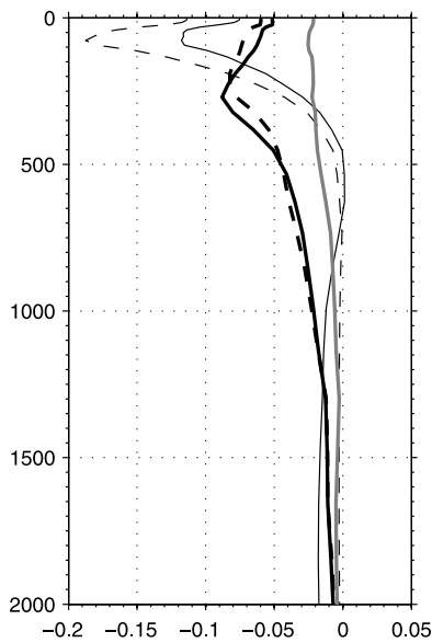
Figure 2. Mean annual salinity averaged along a meridional transect at 20^{\circ}\text{W} (bold line) and 45^{\circ}\text{W} (light line) in experiments NAO (black solid), WIND (black dashed) and (only for 20^{\circ}\text{W} ) WIND-ARCT (grey solid).
