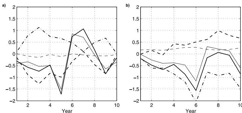
Figure 4. Rate of salinity change (in 10^{-9} psu s^{-1} ) during the 10 years of experiment WIND averaged within (a) the southern box and (b) the northern box indicated in Figure 1: net rate of change (light solid) and contribution from the horizontal advection anomaly (bold solid). Also detailed are contributions to this horizontal advection anomaly due to the Ekman component (light dashed), the anomalous circulation (bold dashed) and the advection of salinity anomaly (bold dashed-dotted). The last two contributions have been divided by 5 in (a).
