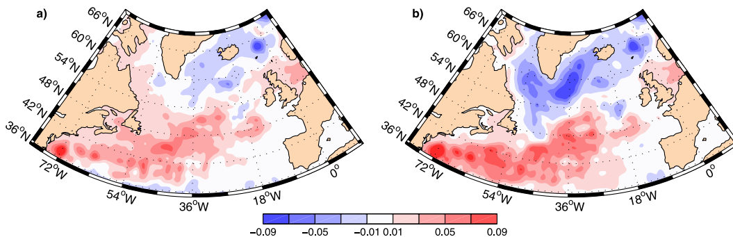
Figure 3. Two-year (year 5 to 6) average of the SSH anomaly (in m) in experiments (a) WIND and (b) NAO.
