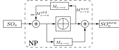
Fig. 2. SO based Node Processor
