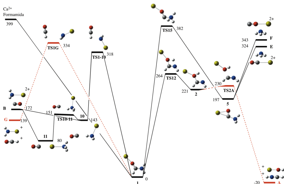
Figure 4. Energy profile of the different reaction mechanisms with origin in the global minimum 1 of the formamide- \text{Ca}^{2+} PES. All values in \text{kJ mol}^{-1} .
