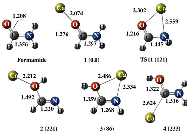
Figure 2. Optimized geometries of the complexes formed by the association of \text{Ca}^{2+} to formamide, formimidic acid and amino(hydroxy)carbene. Relative energies are in \text{kJ mol}^{-1} . The structure of formamide is also included for the sake of comparison.
