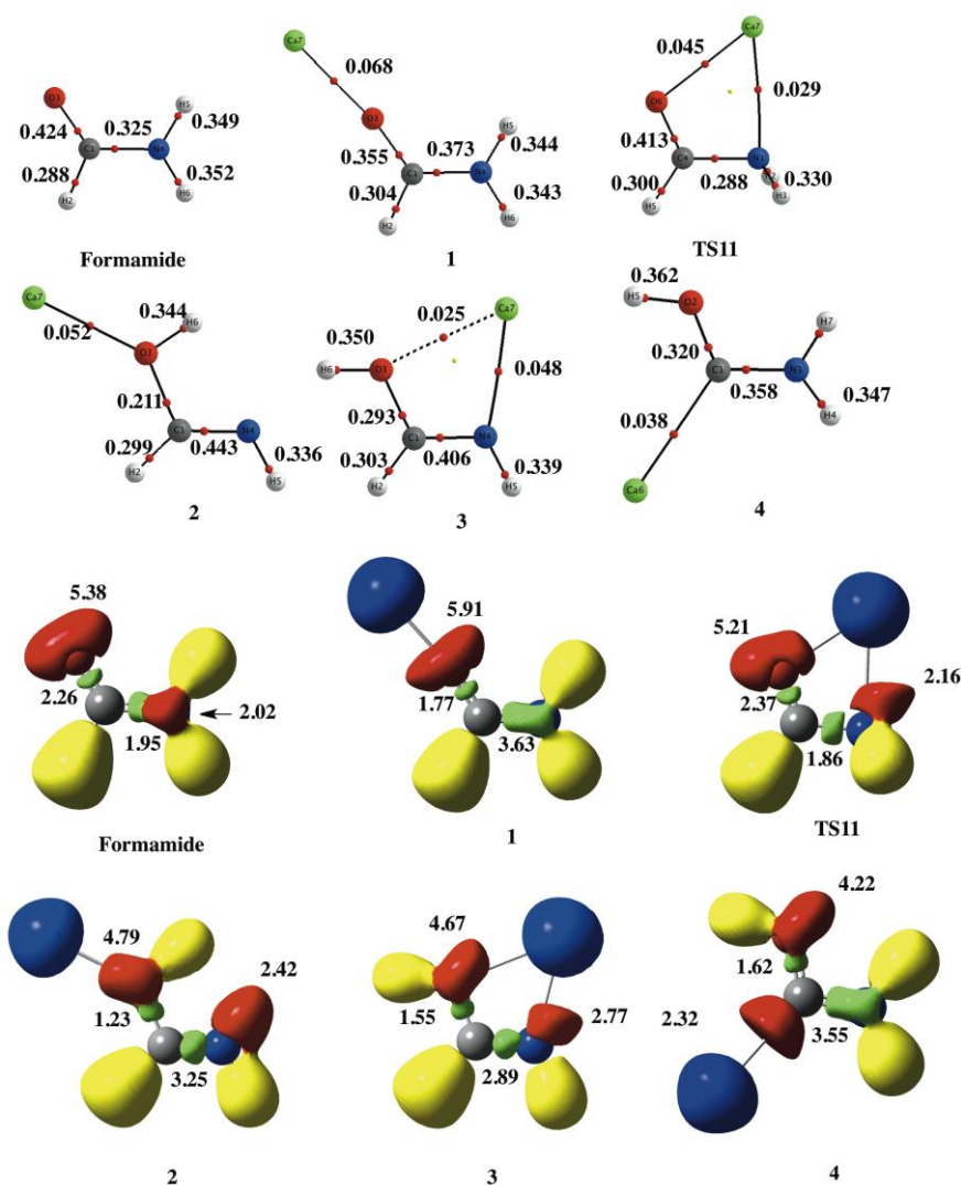
Figure 3. Molecular graphs and ELF plots for the complexes formed by the association of \text{Ca}^{2+} to formamide, formimidic acid and amino(hydroxy)carbene. The structure of formamide is also included for the sake of comparison. In the molecular graphs the red and yellow dots indicate the position of the BCPs and ring critical points, respectively. Electron densities are in a.u.. In the ELF plots the blue, red, and green basins correspond to core-pairs, lone-pairs and bonding-pairs of electrons, respectively. The yellow basins are associated with chemical bonds involving H atoms. The population of the basins are in e^- .
