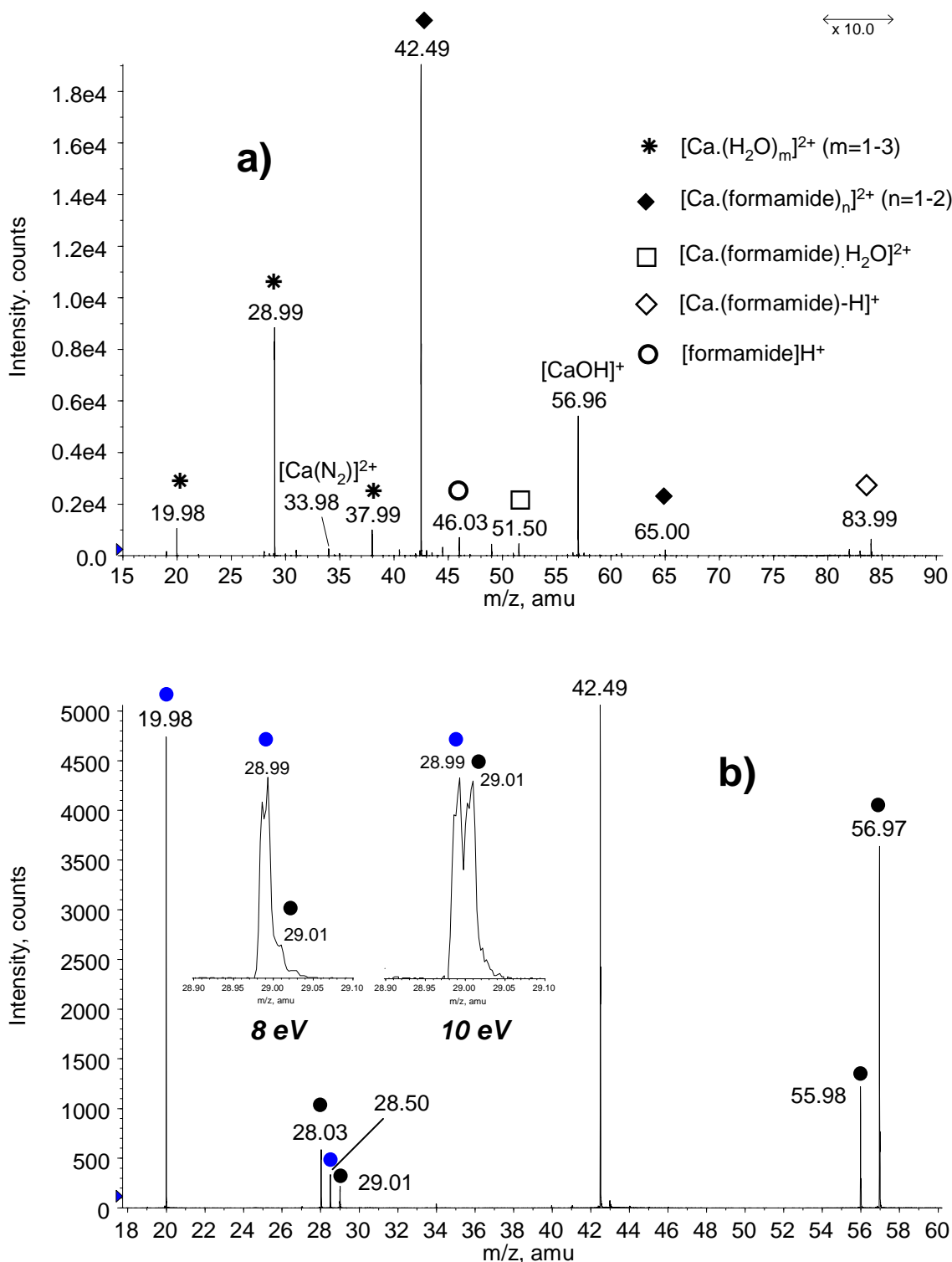
Figure 1: a) Positive nanoelectrospray spectrum of an aqueous CaCl 2 /formamide ( 10^{-3} mol L -1 / 10^{-4} mol L -1 ) mixture, recorded with a declustering potential of 20 V; b) Low-energy CID spectra of the [Ca(formamide)] 2+ complex recorded with a collision energy of 11 eV (laboratory frame), except the insert. See text for details
