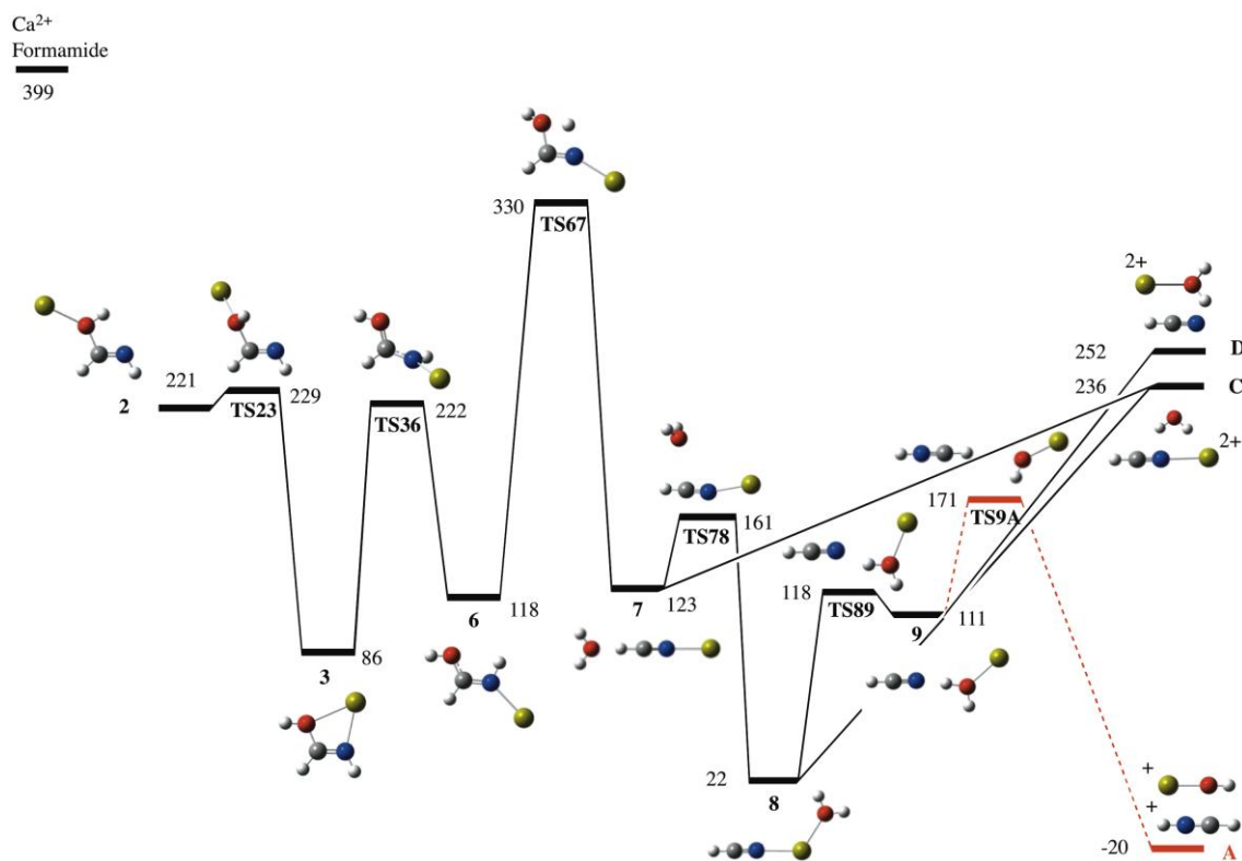
Figure 5. Energy profile of the different reaction mechanism with origin in the local minimum 2 of the formamide-Ca 2+ PES. All values in kJ mol -1 .
