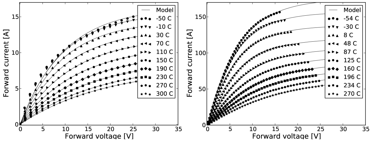
Fig 3: Forward characteristic of a fully-on JFET (i.e V_{gs}=0V ) as a function of the temperature for two JFETs: 2.4x2.4 mm 2 die size (left) and 4x4 mm 2 die size (right). Note that the vertical scales are different.
