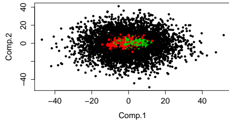
Fig. 1 Simulated data from K = 3 classes (represented by the three colors) of original dimension p = 30 , projected on the PCA axis. We can see that it is a challenging dataset for a clustering algorithm.
