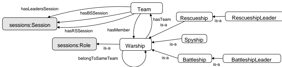
Figure 4: Collaborative Warships application ontology.
