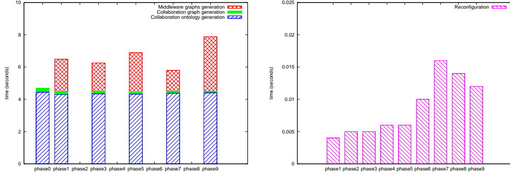
(a) Time elapsed ontology and graphs generation.
