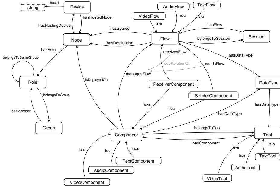
Figure 3: Generic collaboration ontology.
