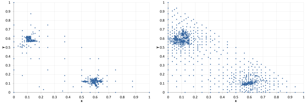
Figure 7: With noise or with overestimated kriging variance: set of simulation points F with noise \sigma_B = 0.1 , s = 0.1 (left) or \sigma_B = 0.1 , s = 1 (right), without re-exploration criterion. w = 0.3 and iterations number is n = 1000 in both cases.
