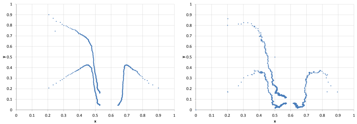
Figure 10: Simulation points with Kiefer-Wolfowitz-Blum algorithm for 2000 points with \sigma_B = 0.1/\sqrt{10} (left), or 20000 points with \sigma_B = 0.1
