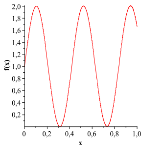
Figure 3: Objective function f(x) = 1 + \sin(15x) + \alpha x , \alpha = 0.01 , without noise.
