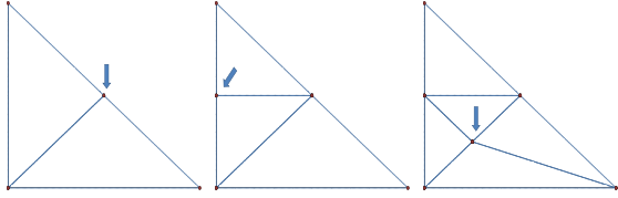
Figure 1: First iterations of a partition of a 2-simplex. Arrows indicate the added observed point at each step.
