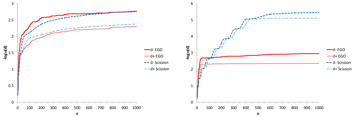
Figure 9: Obtained precisions -\log_{10}(d^-) and -\log_{10}(d^+) after exploration of n points. For EGO (plain red lines, average over 30 runs) and for Scission algorithm (dotted blue lines, average over 1000 runs). Case \sigma_B = 0.1 (left) and \sigma_B = 0 (right).
