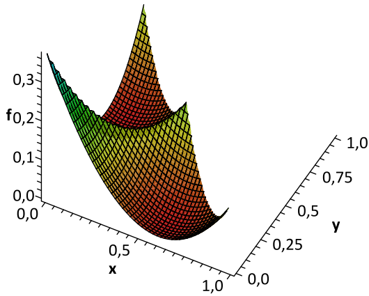
Figure 6: Shape of the function f(\theta) = (\min(x, y) - 0.1)^2 + (\max(x, y) - 0.6)^2 , with \theta = (x, y) .
