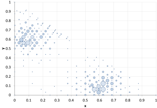
Figure 8: Simulation points for a noise \sigma_B = 0.1 , with re-exploration criterion, (s, w) = (0.1, 0.3) . The number of iterations (exploration or re-exploration) is n = 1000 . The size of bubbles at each explored point \theta = (x, y) are proportional to the number n(\theta) of evaluations of F(\theta) .
