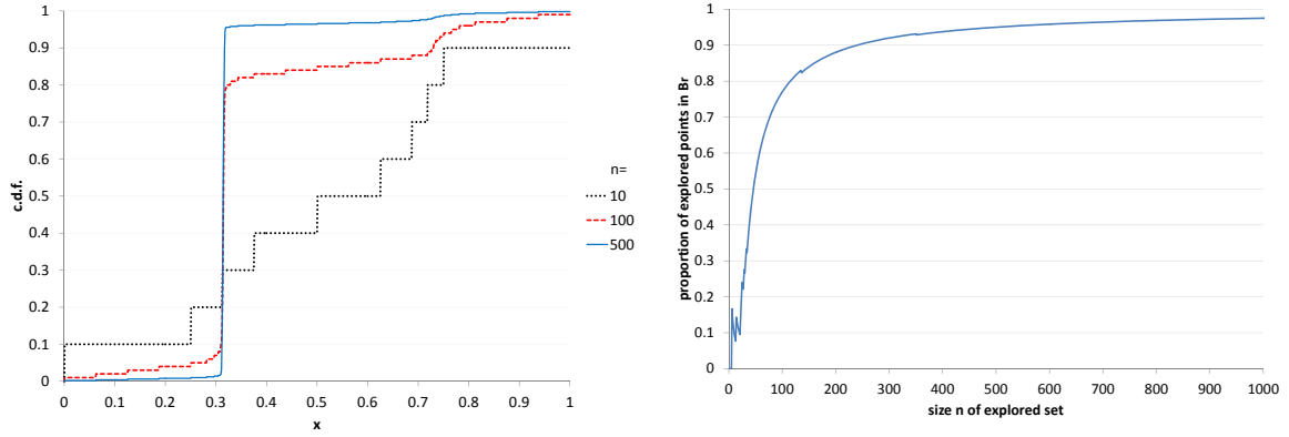
Figure 5: Cumulative distribution function (c.d.f.) of explored points for n = 10 , n = 100 or n = 500 explored points (left) and proportion p_r = \text{card}(\Theta_{\text{obs}} \cap B_r) / \text{card}(\Theta_{\text{obs}}) of points at a given distance to a solution after n = \text{card}(\Theta_{\text{obs}}) explorations (right). Underlying objective function f(x) = 1 + \sin(15x) + \delta x in the case \delta = 0.01 (one global minimizer).
