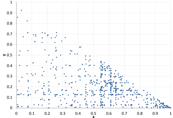
Figure 11: Simulation points with a genetic algorithm for 1000 points with \sigma_B = 0.1
