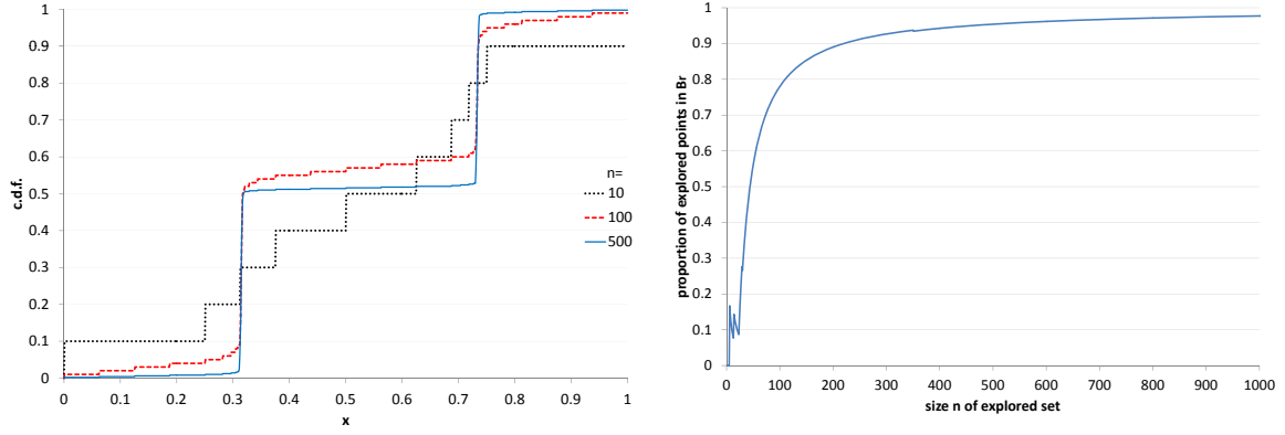
Figure 4: Cumulative distribution function (c.d.f.) of explored points for n = 10 , n = 100 or n = 500 explored points (left) and proportion p_r = \text{card}(\Theta_{\text{obs}} \cap B_r) / \text{card}(\Theta_{\text{obs}}) of points at a given distance to a solution after n = \text{card}(\Theta_{\text{obs}}) explorations (right). Underlying objective function f(x) = 1 + \sin(15x) + \delta x in the case \delta = 0 (two global minimizers).
