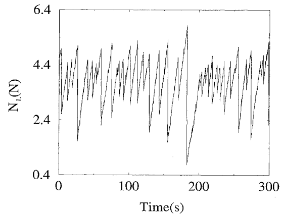
FIG. 3. Typical example of the stick-slip signal observed in experiments, corresponding to variations of the driving force N_L in time.
