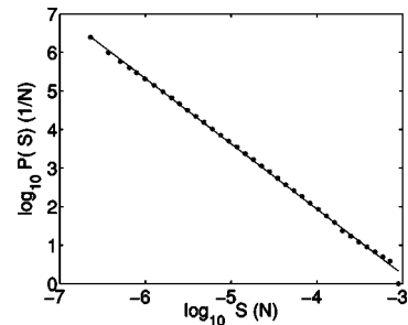
FIG. 6. Probability distribution P of force drops S during slip events. The solid line corresponds to a power law P \propto S^{-b} with b = 1.7 .
