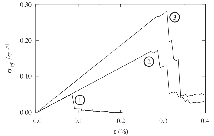
Fig. 3. Stress–strain plots under tensile loading for (1) \sigma^{pm}/\sigma^{[p]} = 0.6 and \rho^m = 0.08 ; (2) \sigma^{pm}/\sigma^{[p]} = 1 and \rho^m = 0.08 ; and (3) \sigma^{pm}/\sigma^{[p]} = 1 and \rho^m = 0.18 .
