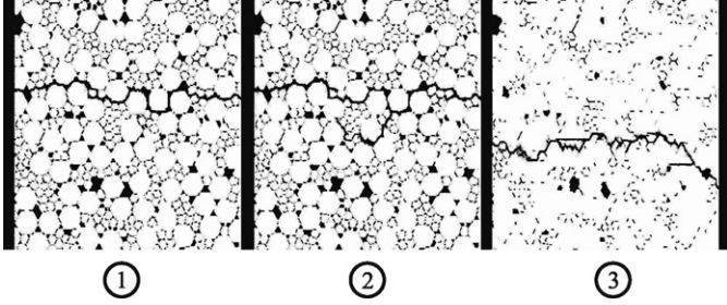
Fig. 4. Crack patterns for (1) \sigma^{pm}/\sigma^{lp} = 0.6 and \rho^m = 0.08 ; (2) \sigma^{pm}/\sigma^{lp} = 1 and \rho^m = 0.08 ; and (3) \sigma^{pm}/\sigma^{lp} = 1 and \rho^m = 0.18 .
