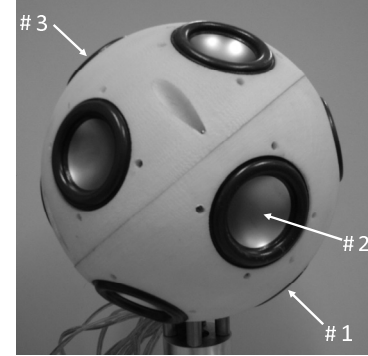
Figure 2: Spherical array prototype with L = 12 independent transducers mounted on a sphere with radius r_e = 0.075 m.
