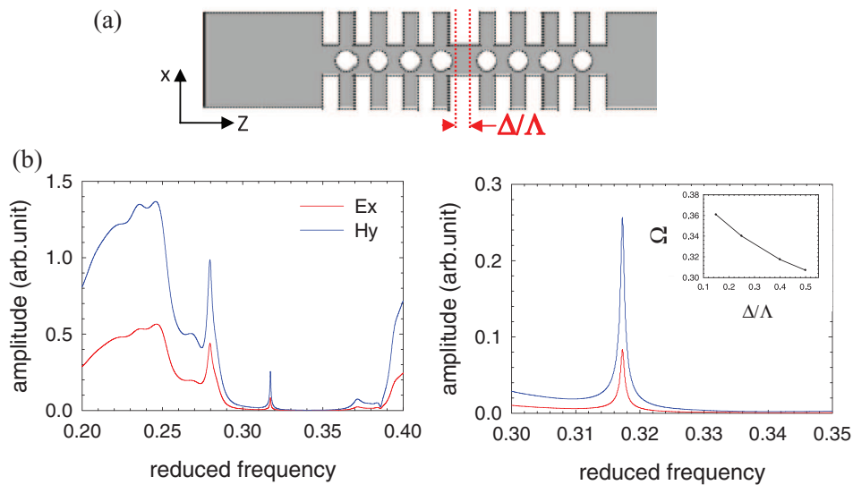
FIG. 6. (a) Schematic view of the (x, z) section of the structure used for the 3D-FDTD calculation of transmission, with \Delta/\Lambda=0.4 . (b) Left: Transmission coefficients for the electric and magnetic fields displaying a resonant peak inside the gap. Right: Magnification of the resonant peak. The inset shows the evolution of the peak frequency as a function of \Delta .
