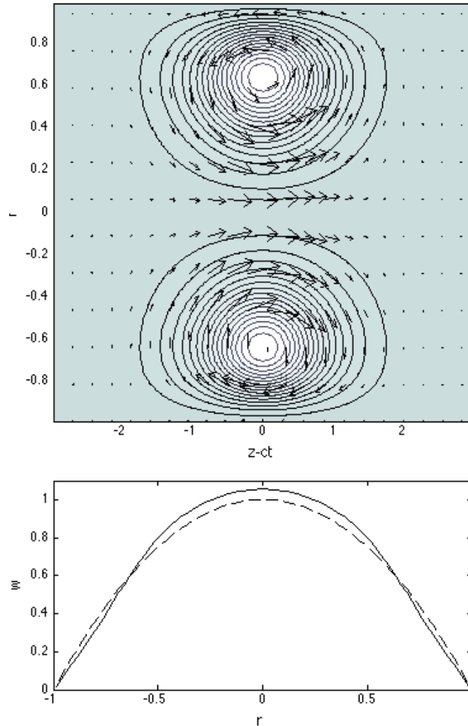
FIGURE 2. Inviscid regular wall vortexon: (top) streamlines of the three-component CH solution of Fig. 1 and (bottom) velocity profiles of the perturbed (solid) and laminar (dash) flows ( c = 0.65 , q = 0 ).
