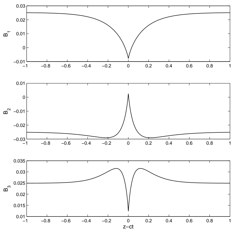
FIGURE 5. Singular vortexon: wave components B_1 , B_2 and B_3 of the CH equations ( c = 0.90 , q = 0.025 ).
