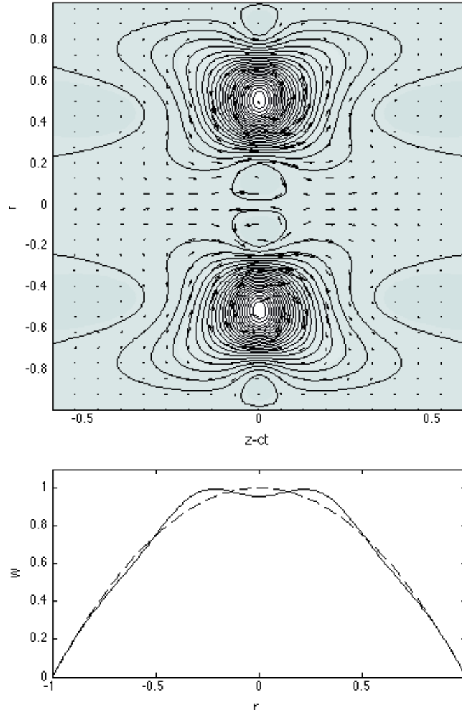
FIGURE 3. Regular wall vortexon: (top) streamlines of the three- component CH solution for c = 0.78 , q = 0 , and (bottom) velocity profiles of the perturbed (solid) and laminar (dash) flows.
