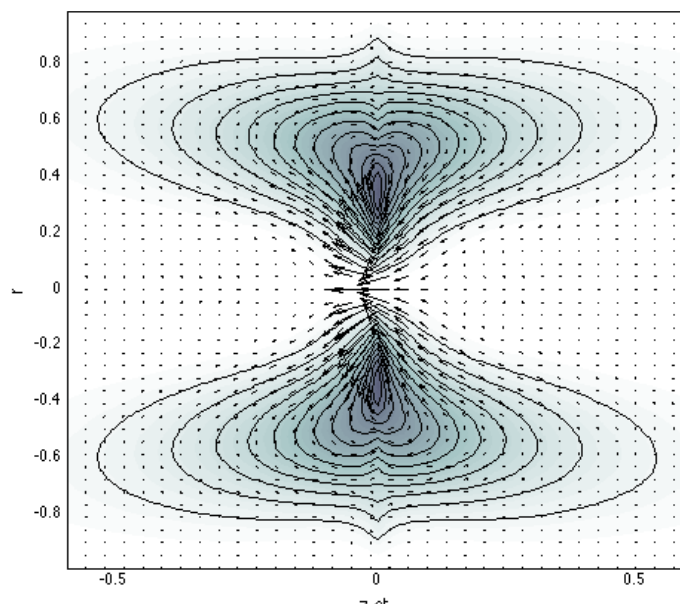
FIGURE 6. Singular vortexon: (top) streamlines of the three- component CH solution of Fig. 5 for c = 0.90 , q = 0.025 , and (bottom) velocity profiles of the perturbed (solid) and laminar (dash) flows.
