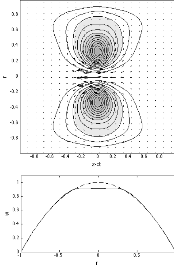
FIGURE 4. Regular centre vortexon: (top) streamlines of the three- component CH solution for c = 0.86 , q = 0 , and (bottom) velocity profiles of the perturbed (solid) and laminar (dash) flows.
