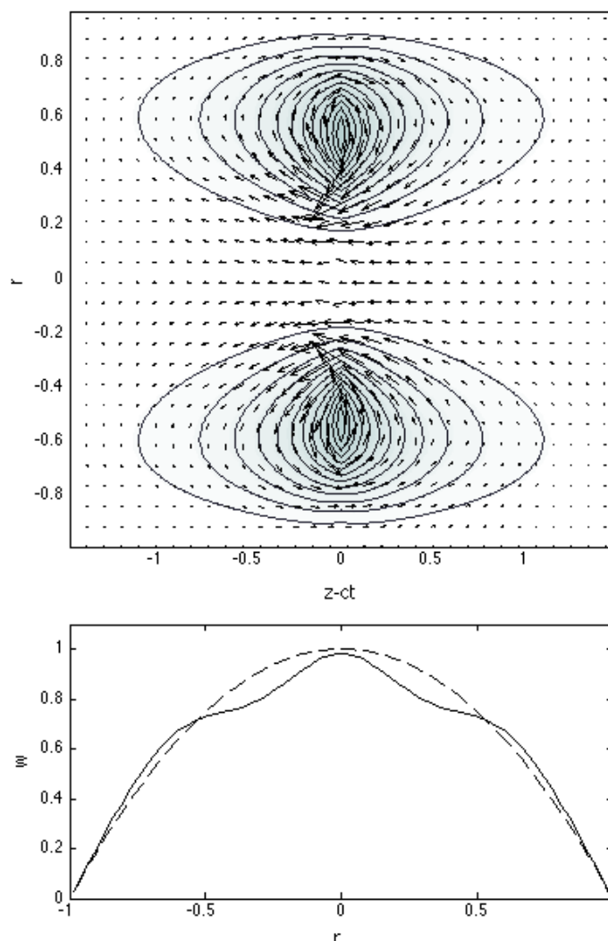
FIGURE 7. Singular vortexon: (top) streamlines of the three- component CH solution for c = 0.70 , q = 0 , and (bottom) velocity profiles of the perturbed (solid) and laminar (dash) flows.
