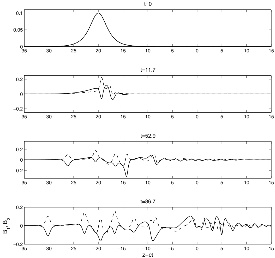
FIGURE 10. Evolution of a perturbation under the CH dynamics: wave components B_1 (solid) and B_2 (dash) at different instants of times ( \text{Re} = 8000 , speed of the reference frame c = 0.75 ).
