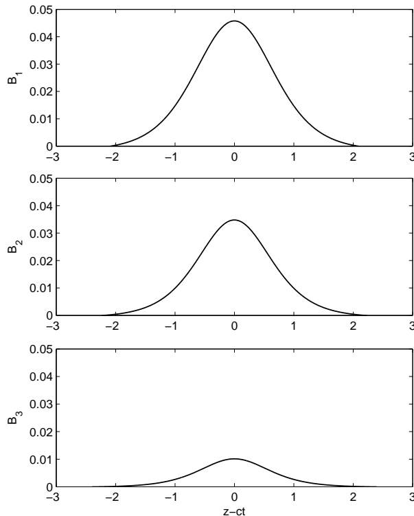
FIGURE 1. Regular wall vortexon: wave components B_1 , B_2 and B_3 of the CH equations ( c = 0.65 , q = 0 ).
