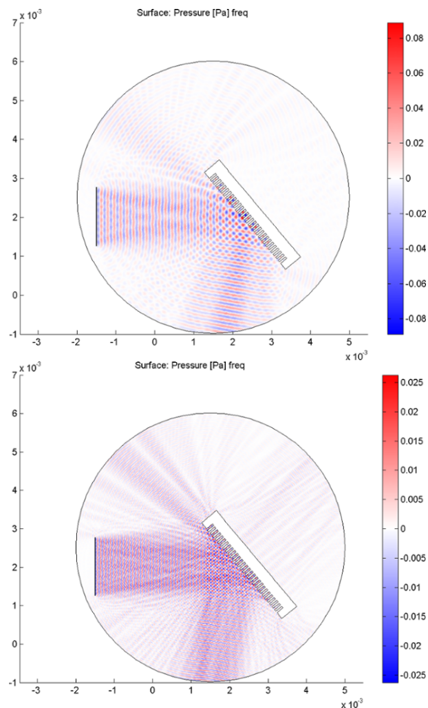
Figure 2: Finite element simulation of diffraction of a plane pressure wave incident on a corrugated silicon plate. Pressure distributions are shown at incidence angle \theta_i = 40^\circ , and frequencies 9 MHz (top) and 18 MHz (bottom). The corrugated silicon plate has parameters a=100 \mu\text{m} and h=200 \mu\text{m} .
