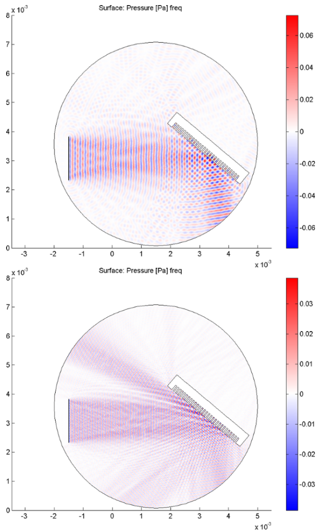
Figure 3: Finite element simulation of diffraction of a plane pressure wave incident on a corrugated silicon plate. Pressure distributions are shown at incidence angle \theta_i = 50^\circ , and frequencies 8.4 MHz (top) and 16.8 MHz (bottom). The corrugated silicon plate has parameters a=100 \mu\text{m} and h=200 \mu\text{m} .
