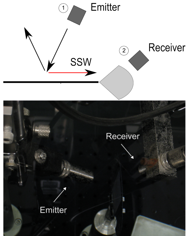
Figure 5: (top) Schematic drawing for diffraction measurements of Scholte-Stoneley waves. (bottom) Photograph of experimental setup showing the sample inside the tank filled with water and the mounts holding the transducers.
