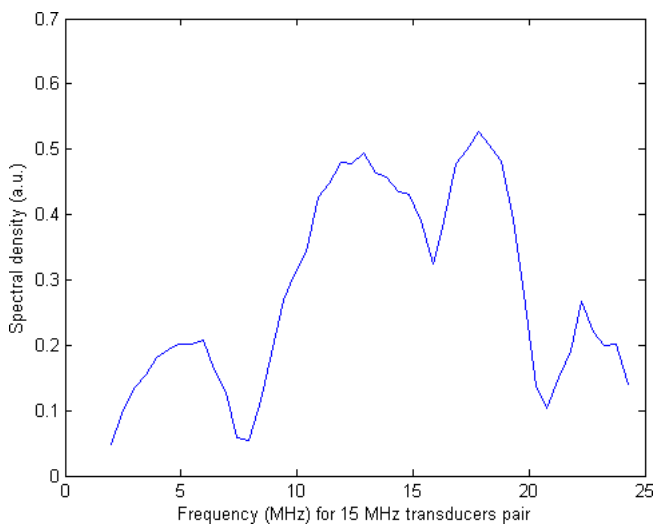
Figure 4: Experimental transmission as a function of frequency (in arbitrary units) for a transducer pair of 15 MHz central frequency.
