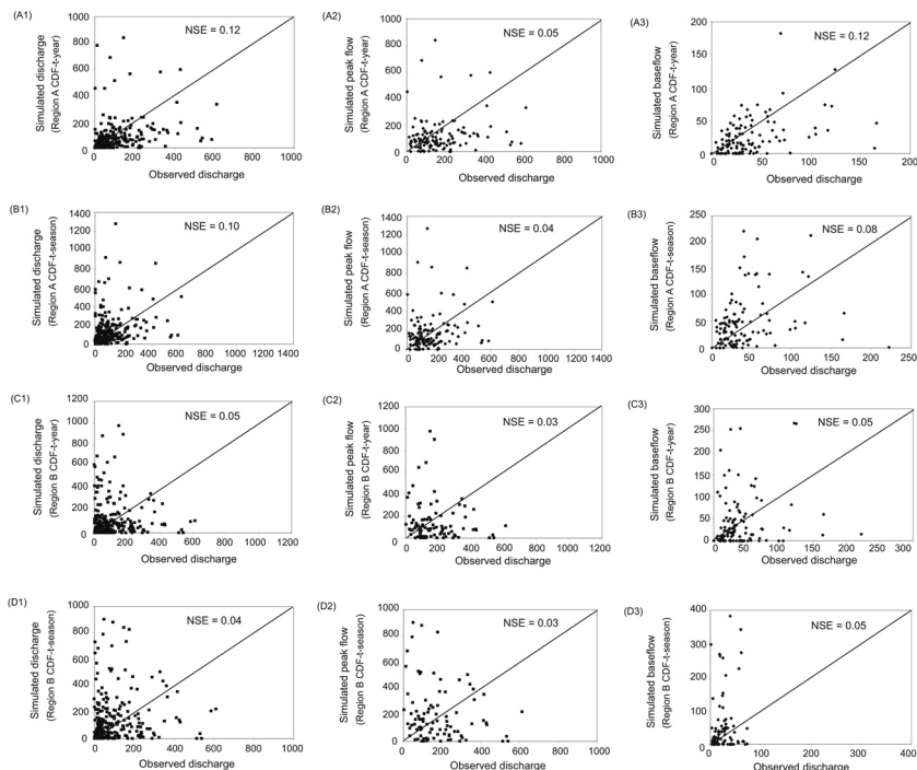
Fig. A5. Scatter plots of measured versus simulated monthly discharge ( \text{m}^3 \text{s}^{-1} ) and the corresponding Nash-Sutcliffe coefficient of efficiency statistic (NSE) over 1950–1972 using (A) downscaled NCEP/NCAR region A by CDF-t-year, (B) downscaled NCEP/NCAR region A by CDF-t-season, (C) downscaled NCEP/NCAR region B by CDF-t-year, and (D) downscaled NCEP/NCAR region B by CDF-t-season.
