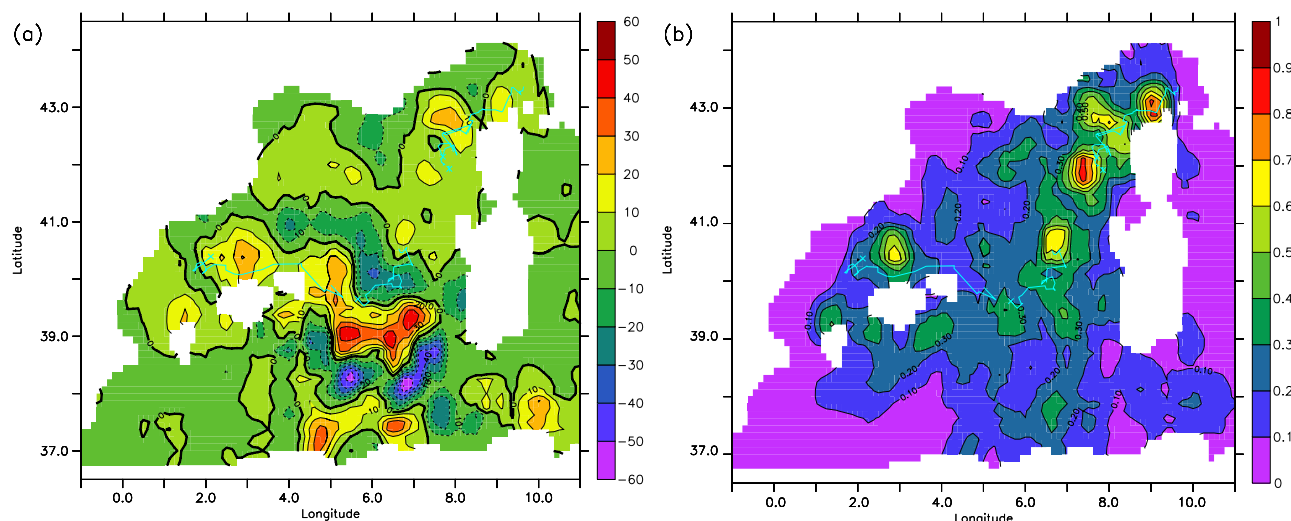
Figure 8. (a) Comparison of the mean EKE as obtained by the two analyzed surface flows over the period 1 January 1 to 31 March 2005. EKEdiff, computed as difference between OStrj and OSref (in \text{cm}^2/\text{s}^2 ), regridded at a 1/8^\circ resolution and low-pass filtered with a cutoff radius of 10 km. The four Argo trajectories are also superimposed. (b) Same as Figure 8a but for EKENorm, computed as absolute EKE difference normalized by the EKE of reference.
