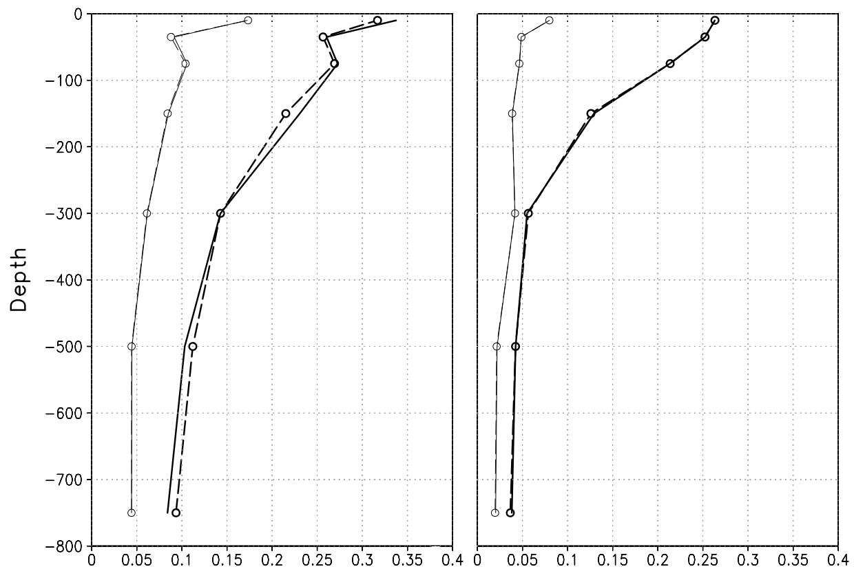
Figure 3. Root mean square of (left) temperature misfits (°C) and (right) salinity misfits (psu) in the period January–March 2005. The two diagnostics AmO (thin lines) and BmO (bold lines), defined in section 3.4, are represented by solid lines for OSref (without trajectory assimilation) and by dashed line for OStrj (with trajectory assimilation).
