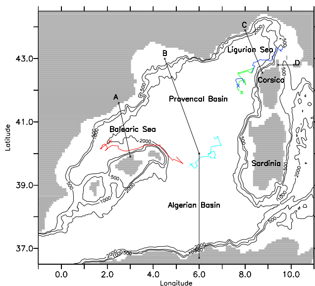
Figure 1. Trajectories of four Argo floats inside the NW Mediterranean. The four sections of the Balearic Sea (section A), the Algero-Provençal basin (section B), the Ligurian Sea (section C), and Corsica Channel (section D) are also indicated by lines superimposed on the isobaths 500, 1000, and 2000 m.
