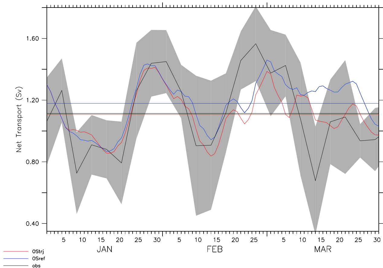
Figure 9. Evolution of the net transport crossing the section of the Corsica Channel. Plot in blue corresponds to OSref, plot in red corresponds to OStrj, and plot in black corresponds to the independent observation by moored current meter. The envelope of admissible values with respect to the standard deviation of the observed transports is indicated by gray shading. The mean transports over the period are also plotted by the horizontal lines. The time series from the two analyses have been low-pass filtered with a cutoff period of 4 days.
