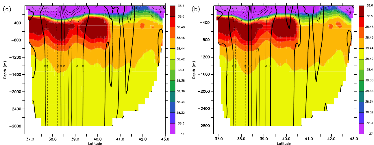
Figure 5. (a) Mean stratification along the section B (Algero-Provençal basin). Salinity (in psu) extracted daily from the analysis OSref, and averaged during the period 1 January 1 to 31 March 2005. Contours are absolute velocities normal to the section (in cm/s, every 5 cm/s) averaged over the same period. (b) Same as Figure 5a but for the analysis OStrj.
