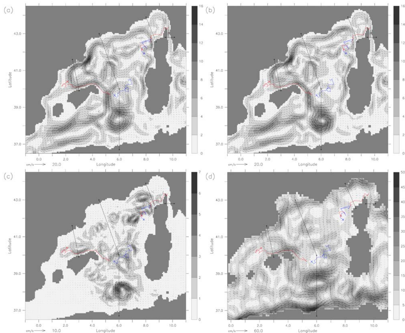
Figure 4. (a) Mean circulation at 350 m computed from OSref. The velocities (in cm/s) are superimposed on the amplitude (in cm/s) of the currents, as well as the four Argo trajectories and the four sections. (b) Same as Figure 4a but for the mean circulation at 350 m computed from OStrj. (c) Same as Figure 4a but for the difference between the two flows at 350 m (OStrj – OSref). (d) Same as Figure 4a but for the mean circulation computed from currents reconstructed by sea surface topography (Aviso product).
