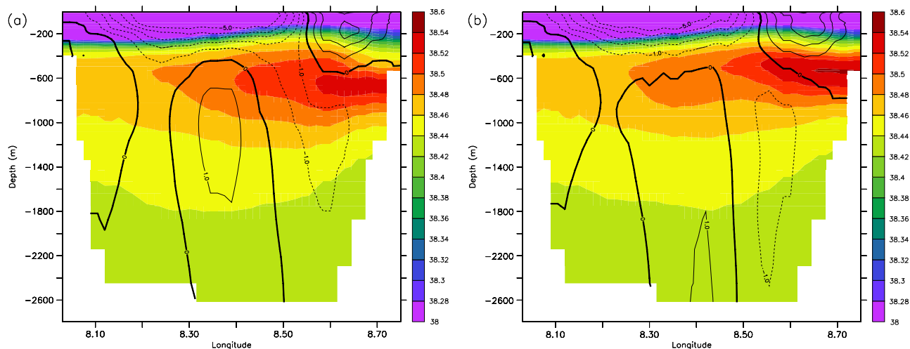
Figure 7. (a) Same as Figure 5a but along the section C (Ligurian Sea). Contours are absolute velocities normal to the section (in cm/s, every 1 cm/s) averaged over the same period. (b) Same as Figure 7a but for the analysis OStrj.
