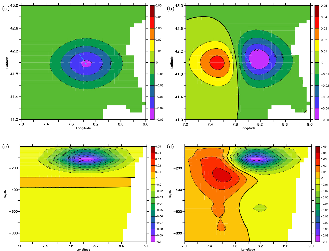
Figure 2. (a) Structure of the correction term provided by single observation experiments in the neighborhood of Corsica. Difference between the salinity (in psu) analyzed with a TS profile located at ( 42^{\circ}\text{N} , 8^{\circ}\text{E} ) and the background salinity field at 200 m; the Argo drift at 350 m is superimposed. (b) Same as Figure 2a but considering the analysis of the same TS profile plus the subsurface drift. (c) Same as Figure 2a but along a zonal section at 42^{\circ}\text{N} . (d) Same as Figure 2b but along a zonal section at 42^{\circ}\text{N} .
