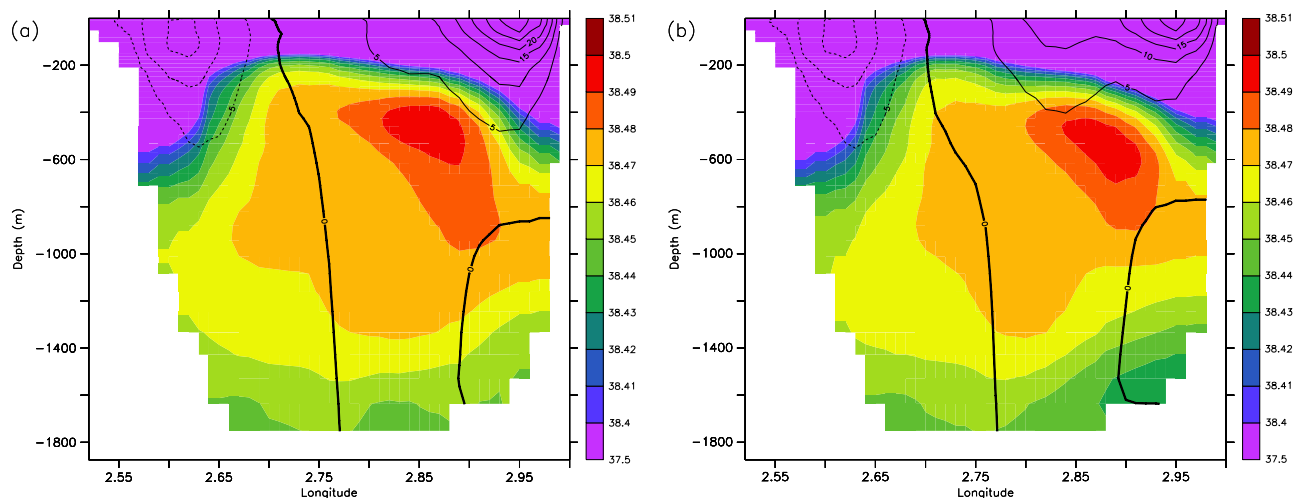
Figure 6. (a) Same as Figure 5a but along the section A (Balearic Sea). (b) Same as Figure 6a but for the analysis OStrj.
