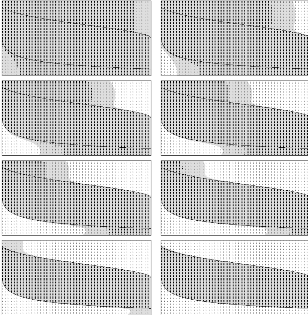
Fig. 1. Example of progressive approximation of the viability kernel in 2 dimensions for the population problem. The horizontal axis represents the population size ( x ) and the vertical axis its evolution rate ( y ). K is the rectangle which limits the points of the grid. The grid includes 2601 points (51 points per dimension). The dark points of the grid are the ones belonging to K_h^{n+1} . The approximation of the kernel L(K_h^n) is represented in gray. The parameter dt is computed for defining moves of size 2\beta(h) in one time step and the optimisation is made on 10 time steps.
