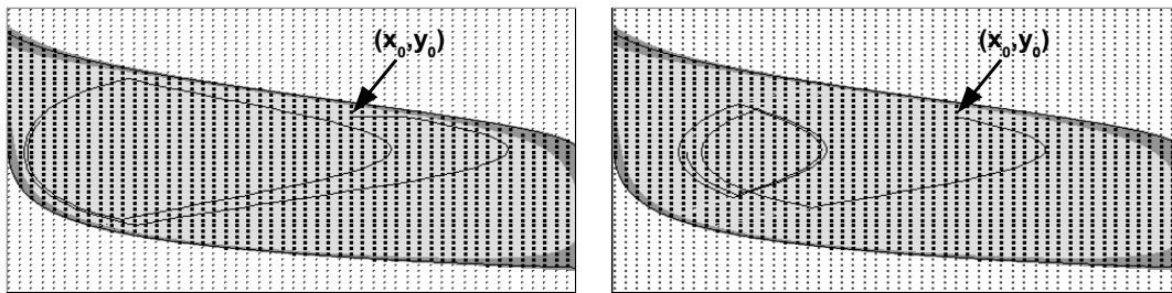
Fig. 3. Example of heavy trajectories from a point (x_0, y_0) . The difference between L(K_h^p) and A_\Delta is in dark gray. The trajectories include 200 time steps. On the left: 2 time steps anticipation. On the right: 8 time steps anticipation.
