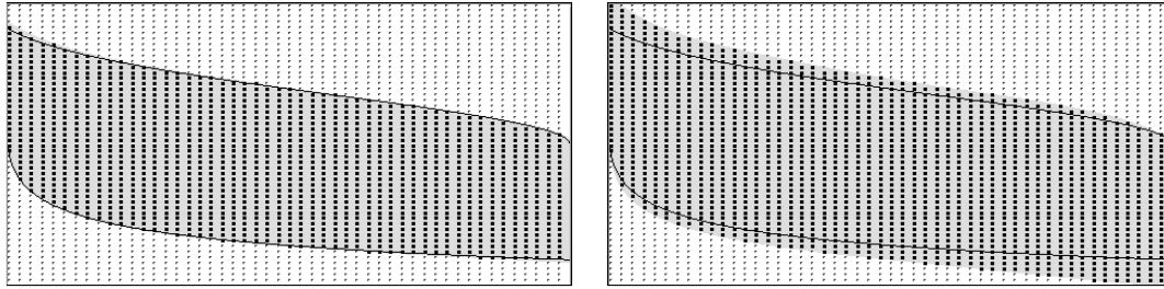
Fig. 2. Comparison of the final approximation of the viability kernel for optimisations with different time steps: On the left, the control optimisation is made on 1 time step and on the right on 10 time steps. dt is computed for defining moves of size 2\beta(h) in one time step.
