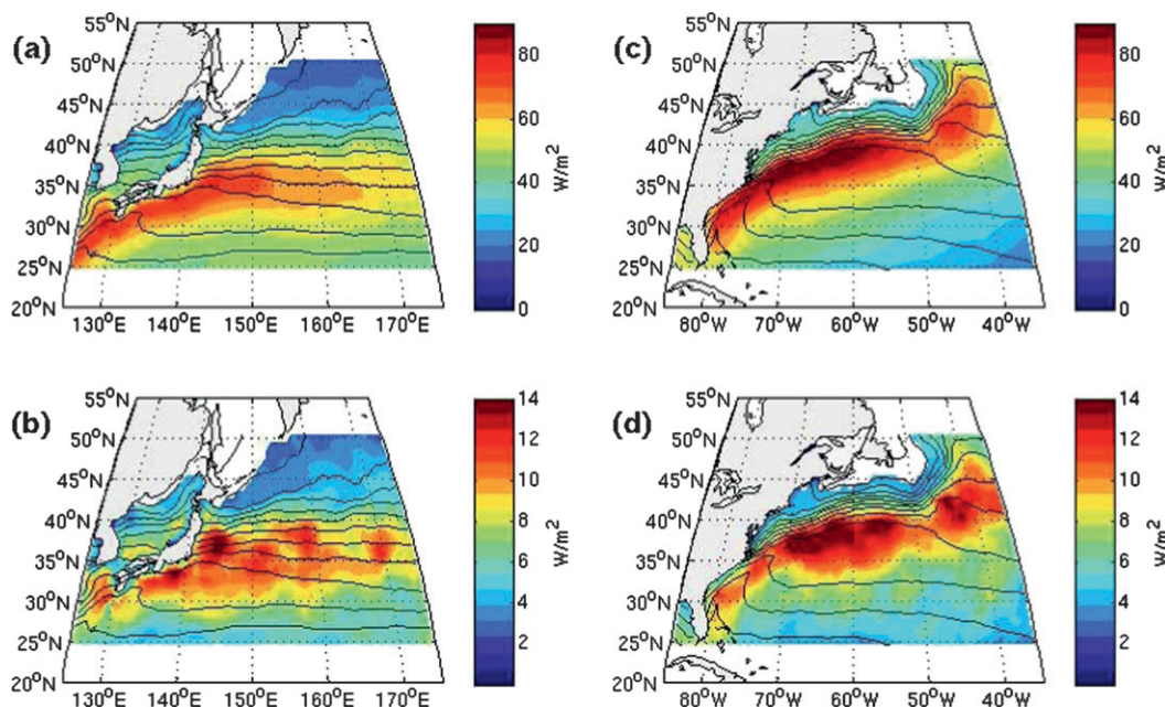
FIG. 13. (a) The 22-yr mean of each winter's (JFM) standard deviation of the 2–8-day bandpass-filtered daily latent heat flux from the objectively analyzed air–sea fluxes (OAF flux) for 1983–2004 (Yu et al. 2008). Contours are the climatological mean winter (JFM) SST with 2°C interval. (b) Interannual standard deviation of each winter (JFM)'s standard deviation of the 2–8-day bandpass-filtered daily latent heat flux. (c),(d) As in (a),(b), but for the North Atlantic. The figure is reproduced from Figs. 7 and 12 of Joyce et al. (2009).
