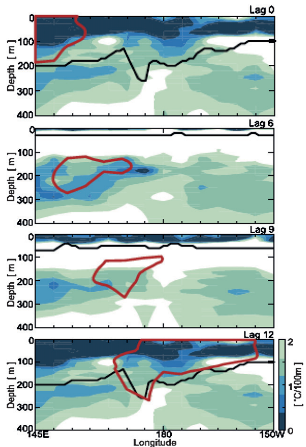
FIG. 6. Vertical sections showing reemergence of SST anomalies over the North Pacific along the line between 30^{\circ}\text{N} , 145^{\circ}\text{E} and 34^{\circ}\text{N} , 150^{\circ}\text{W} . Red lines indicate domains where the correlation coefficients of subsurface temperature anomalies with a reference index exceed 0.7 for lags of (top to bottom) 0, 6, 9, and 12 months. The index has been defined as winter-mean SST anomalies averaged over 27^{\circ} – 33^{\circ}\text{N} , 137^{\circ} – 154^{\circ}\text{E} . Color shading represents the strength of vertical temperature gradient [ ^{\circ}\text{C}/(100\text{m})^{-1} ], as indicated on the right. Black lines denote the mixed layer bottom. (After Sugimoto and Hanawa 2005.)
