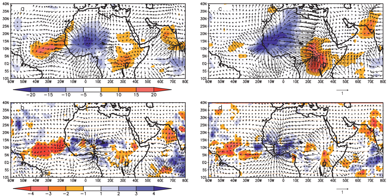
FIG. 7. (a) Strong minus weak convective events at t_0 for June–September 1979–2006 based on the reconstructed 10–30-day filtered OLR ITCZ index by S-EOF1 and S-EOF2: unfiltered OLR values (colors; units: \text{W m}^{-2} ), and 200-hPa divergent wind vectors ( \text{m s}^{-1} ). (b) As in (a), but for the unfiltered GPCP values over the period 1997–2006 (colors; \text{mm day}^{-1} ) and 700-hPa divergent wind vectors ( \text{m s}^{-1} ). (c) As in (a), but for the reconstructed 10–30-day filtered OLR ITCZ index by S-EOF2, S-EOF3, and S-EOF4. (d) As in (b), for the reconstructed 10–30-day filtered OLR ITCZ index by S-EOF2, S-EOF3, and S-EOF4. Color scale is the same for (a) and (c), and for (b) and (d). Vector scale is the same for all the panels.
