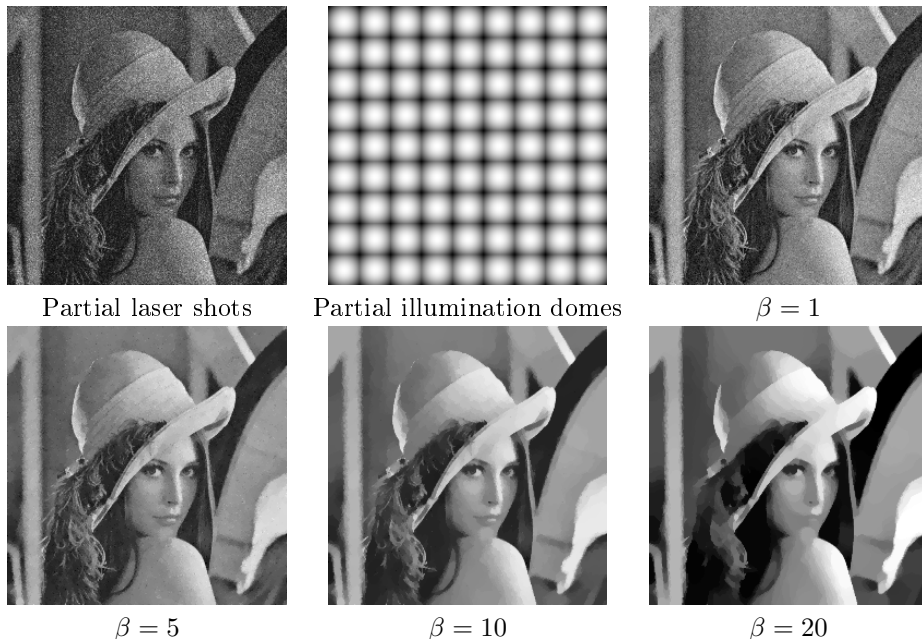
FIGURE 3. Reconstruction with a noise level \sigma = 0.1 . The remaining parameters are set with \sigma_c = 10^{-4} , \sigma_w = 10^{-4} and \bar{w} = 30 . Each pixel of the top left and middle top images is assigned with its maximum intensity over all k \in \{1, \dots, K\} . Then we present the results for different \beta .
