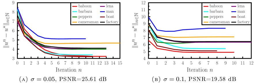
FIGURE 5. Convergence of the algorithm of Table 3 for two noise levels. On each figure, the distance between the image estimate u^n and the true image u^* is represented as a function of the iteration n . The PSNR between the noisy and the noise-free laser shots is also indicated as a measure of the difficulty of the problem. The remaining parameters are set as follows: \bar{w} = 16.2 , \sigma_c = 0.81 and \sigma_w = 0.07 .
