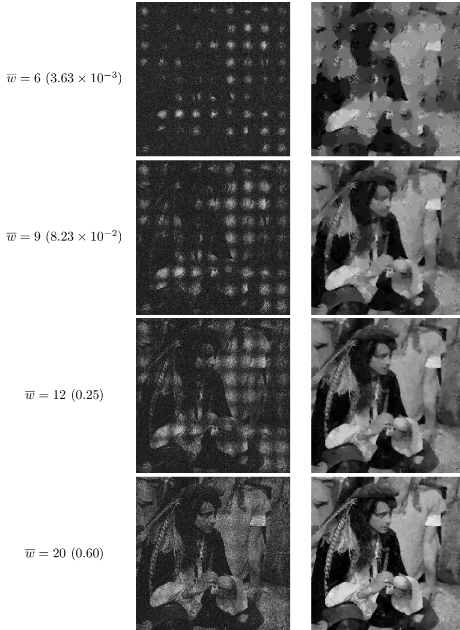
FIGURE 4. Influence of the parameter \bar{w} on the reconstruction with a noise level \sigma = 0.1 . The remaining parameters are set to \sigma_c = 10^{-4} and \sigma_w = 10^{-4} . On the middle column, each pixel of the images is assigned with its maximum intensity over all laser shots k \in \{1, \dots, K\} . On the right column, we provide the results of the algorithm of Table 3. As a measure of the difficulty of the problem, we also provide, next to \bar{w} , the quantity (14) within parenthesis.
