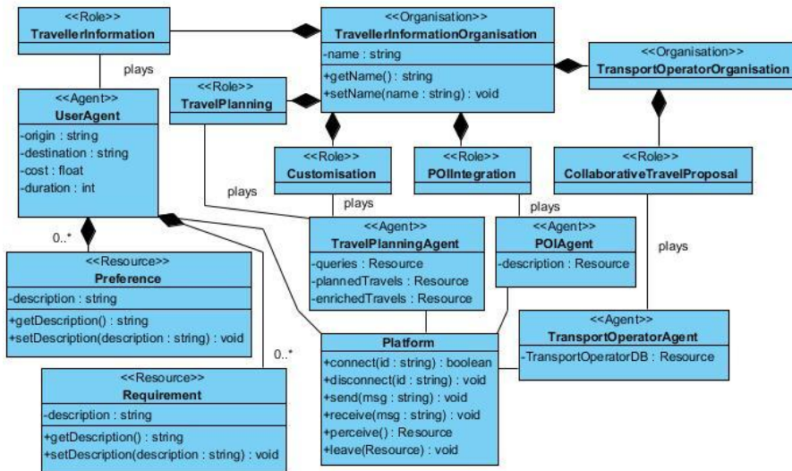
Fig. 4. Instantiation of the “Platform-based System Architecture” AgentDesign Pattern
