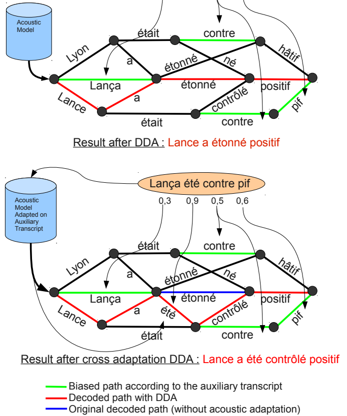
Fig. 4. Cross adaptation and DDA examples at the graph level.
