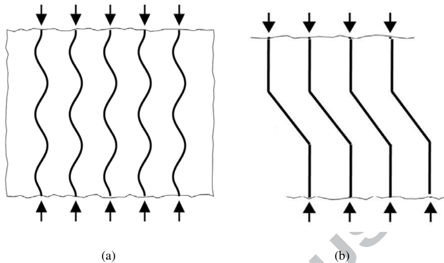
Figure 1: Schematics of the two major deformation modes proposed for fibre composite materials: In (a), deformation is accommodated by in-phase microbuckling of the fibres as predicted by Rosen [4], (b) shows a direct fibre deflection into a kinked shape according to Argon [10]
