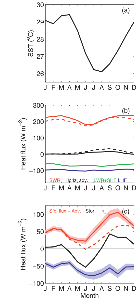
FIG. 4. Area-averaged seasonal cycles in the SCTR region: (a) SST; (b) surface SWR (solid red line), SWR absorbed in the mixed layer (dashed red line), zonal advection (solid black line), meridional advection (dashed black line), the sum of net longwave radiation and sensible heat flux (green line), and latent heat flux (blue line); and (c) the sum of the net surface heat flux and horizontal advection (solid red line), net surface heat flux (dashed red line), mixed layer heat storage rate (black line), and heat balance residual (blue line). Shading in (c) represents one standard error.
