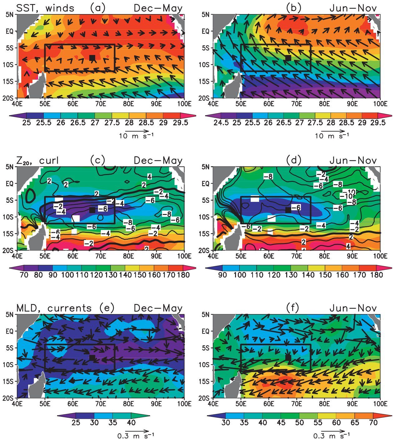
FIG. 1. Climatological (2000–07) SST (shaded; ^{\circ}\text{C} ) and surface wind vectors during (a) December–May and (b) June–November. The box encloses the SCTR region, and the solid black square is the position of the 8^{\circ}\text{S} , 67^{\circ}\text{E} RAMA mooring. (c),(d) As in (a),(b), but for thermocline depth as inferred from the 20^{\circ}\text{C} isotherm (shaded; m) and wind stress curl (contours; 10^{-5} \text{ N m}^{-3} ). (e),(f) As in (a),(b), but for MLD (shaded; m) and surface current vectors.
