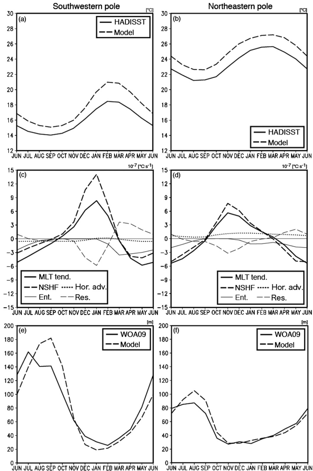
FIG. 3. Seasonal cycle of (a),(b) SST ( ^{\circ}\text{C} ), (c),(d) each term in Eq. (1) ( 10^{-7} \text{ }^{\circ}\text{C s}^{-1} ), and (e),(f) mixed layer depth (m) at the southwestern and northeastern poles of the IOSD defined in Fig. 2b. In (a),(b) the SSTs from HADISST (solid line) and SINTEX-F model (dashed line) are shown. In (c),(d) the mixed layer temperature tendency (MLT tend., thick solid line), net surface heat flux (NSHF, thick dashed line), horizontal advection (Hor. adv., thick dotted line), entrainment (Ent., thin solid line) and residual (Res., thin dashed line) terms are shown. In (e),(f), the mixed layer depths derived from WOA09 (solid line) and the model (dashed line) are shown.
