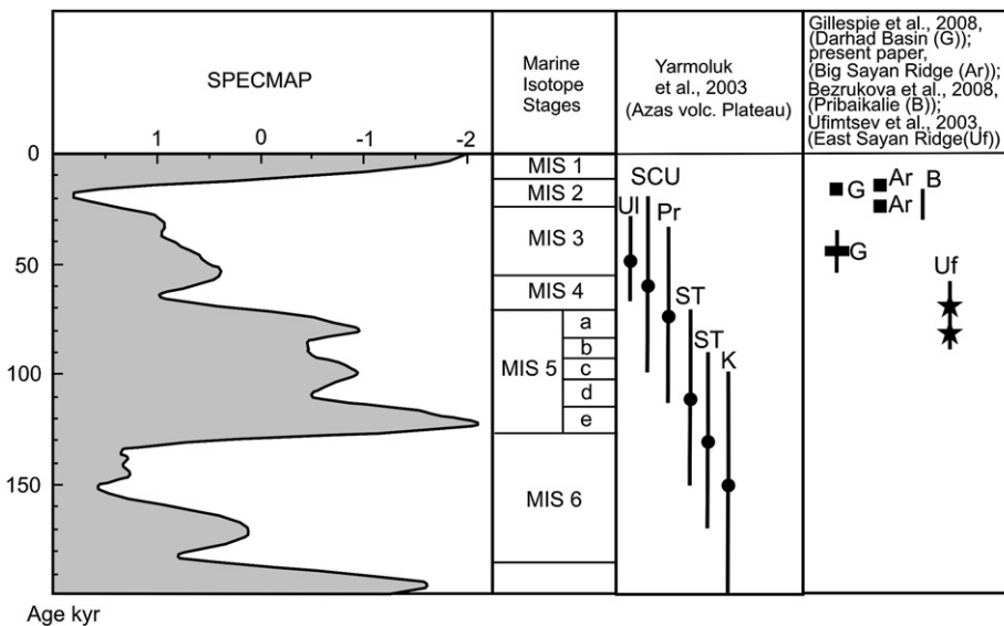
Fig. 13. K/Ar dates for subglacial volcanoes (black circles), exposure ages of Darhad Basin and Big Sayan Ridge (black squares), 14 C, IRSL, OSL dates of Darhad Basin – black rectangle, pollen and AMS dates of Pribaikalie (black line) and RTL dates of East Sayan Ridge (black stars). Ul – Ulug-Arginskii; SCU – Sorug-Chushku-Uzu; Pr – Priezernyi; ST – Shivit-Taiga; K – Kokhemskii.
