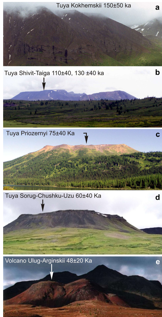
Fig. 8. Field photographs showing the volcanoes formed on the Azas volcanic Plateau. (a, b, c, d) volcanoes erupted through ice cap. (e) Ulug-Arginskii volcano formed in the aerial environment.
