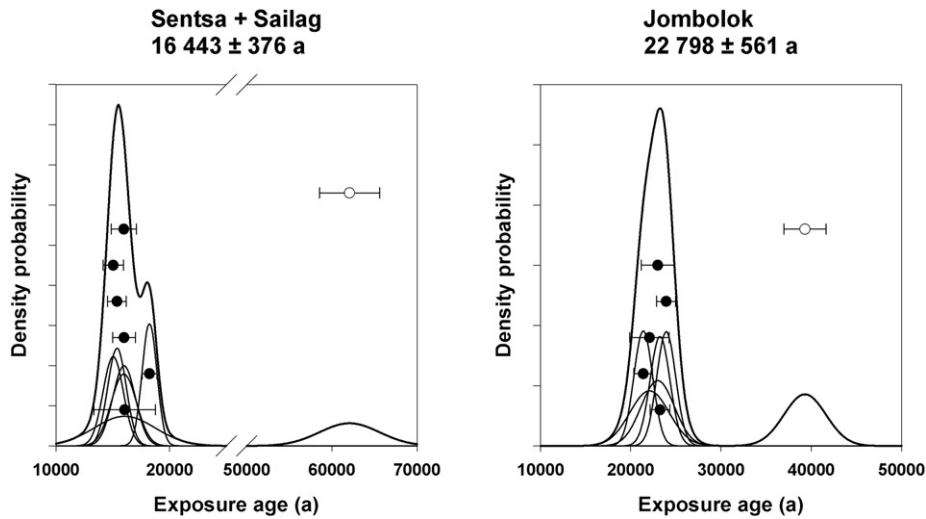
Fig. 12. Cosmogenic 10 Be weighted mean exposure ages.
