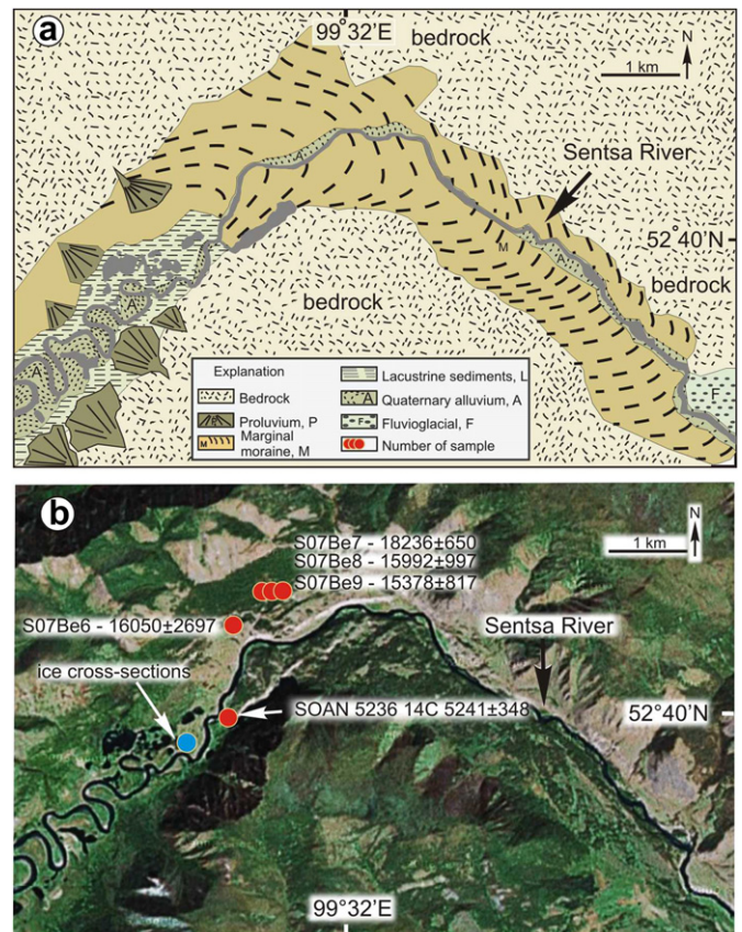
Fig. 6. Sentsa terminal moraine. (a) Schematic drawing of the Quaternary deposits. (b) Fragment of the Landsat satellite image with references to sampling sites and ^{10}\text{Be} and ^{14}\text{C} ages. Blue circle is the buried ice discovered in the Sentsa River valley. (For interpretation of the references to color in this figure legend, the reader is referred to the web version of this article.)
