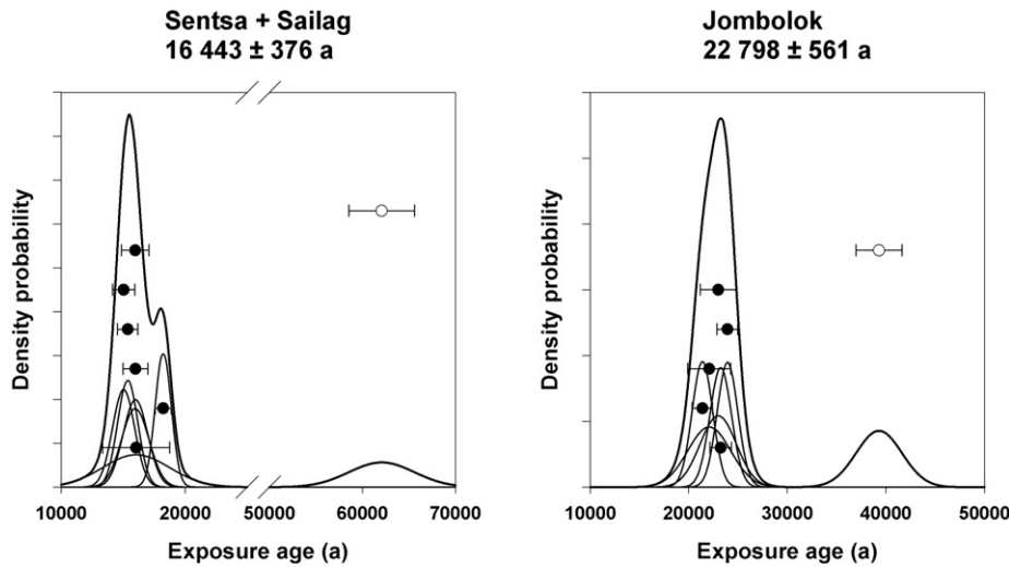
Fig. 12. Cosmogenic ^{10}\text{Be} weighted mean exposure ages.
