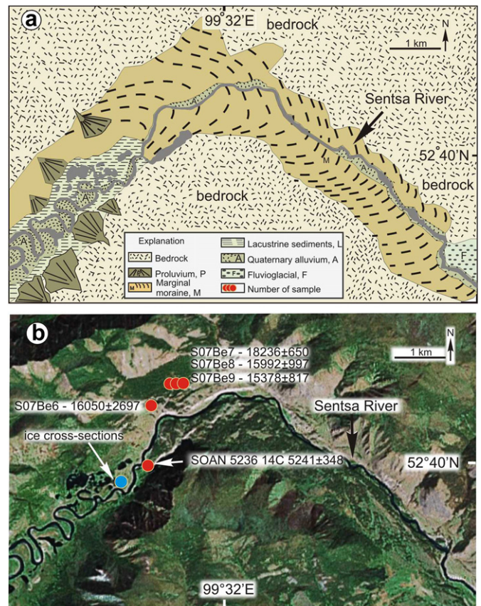
Fig. 6. Sentsa terminal moraine. (a) Schematic drawing of the Quaternary deposits. (b) Fragment of the Landsat satellite image with references to sampling sites and 10 Be and 14 C ages. Blue circle is the buried ice discovered in the Sentsa River valley. (For interpretation of the references to color in this figure legend, the reader is referred to the web version of this article.)
