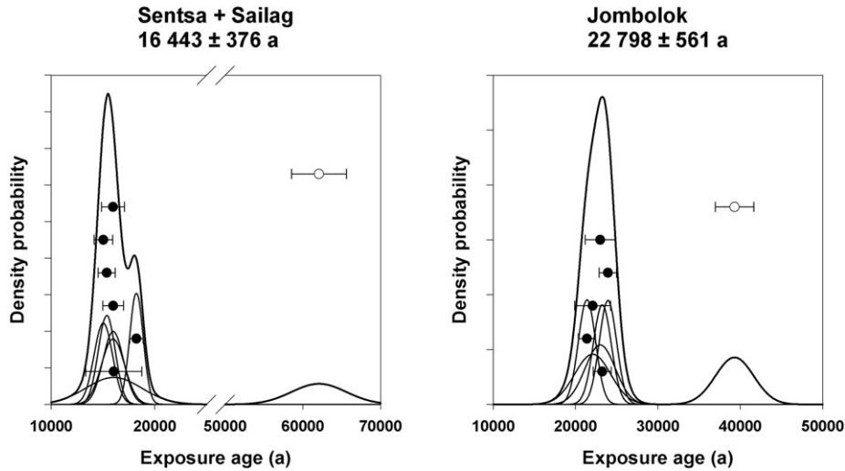
Fig. 12. Cosmogenic ^{10}\text{Be} weighted mean exposure ages.
