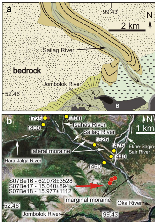
Fig. 5. Sailag marginal moraines. (a) Schematic drawing of Quaternary deposits. (b) Fragment of the Landsat satellite image with references to sampling sites and 10 Be ages. The yellow circles indicate the altitudes of the lateral moraines. (For interpretation of the references to color in this figure legend, the reader is referred to the web version of this article.)
