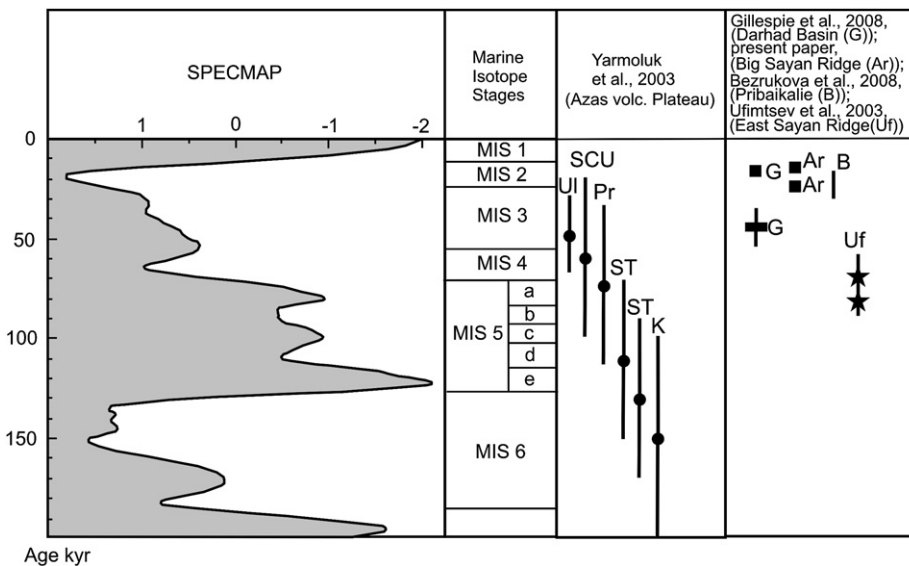
Fig. 13. K/Ar dates for subglacial volcanoes (black circles), exposure ages of Darhad Basin and Big Sayan Ridge (black squares), ^{14}\text{C} , IRSL, OSL dates of Darhad Basin – black rectangle, pollen and AMS dates of Pribaikalie (black line) and RTL dates of East Sayan Ridge (black stars). Ul – Ulug-Arginskii; SCU – Sorug-Chushku-Uzu; Pr – Priezernyi; ST – Shivit-Taiga; K – Kokhemskii.
