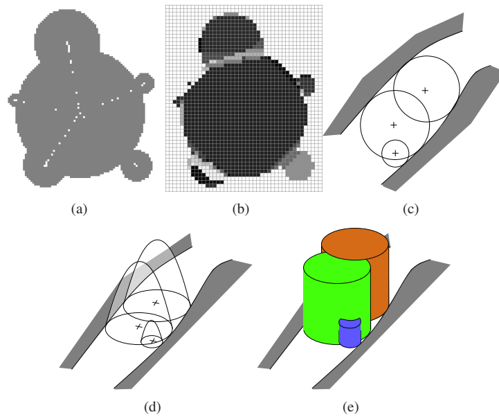
Figure 2: Discrete medial axis (a) and discrete power diagram of a 2D shape (b, one gray value color per power cell). Given a subset of three maximal balls i \in \{1, 2, 3\} (c), illustration of \{x, \sigma'_i(x)\} (d) and \{x, h_i(x)\} (e) surfaces.
