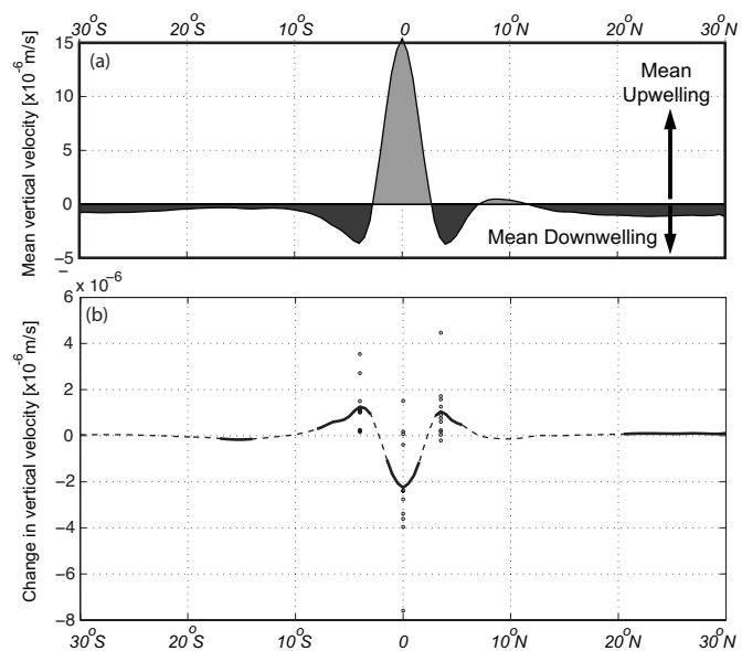
Fig. 7 a) Vertical velocities of water ( 10^{-6} \text{ m.s}^{-1} ) at a depth of 50 m, for 1990 (mean 1980 – 1999), averaged between 170°E and 110°W, where a positive velocity corresponds to upwelling and a negative velocity to downwelling; and b) Climate driven changes to vertical velocities for 2100 (full line if significant at 95%; dashed line otherwise). Values for individual CMIP3 models are indicated in the maxima (small circles). The strong equatorial upwelling shows decreases that are immediately balanced by strong downwelling near 4°N–4°S so that net upwelling between 9°S and 9°N does not change.
