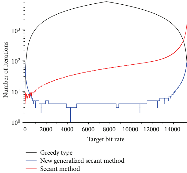
FIGURE 3: Number of iterations of the secant and generalized secant methods, and greedy-type algorithm versus the target bitrate, n = 1024 , r_{\max} = 15 .
