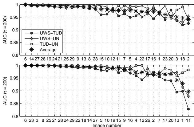
Fig. 9. Impact of the image content measured using AUC ( \tau = 200 ) for t = 1 s (top) and t = 10 s (bottom).
