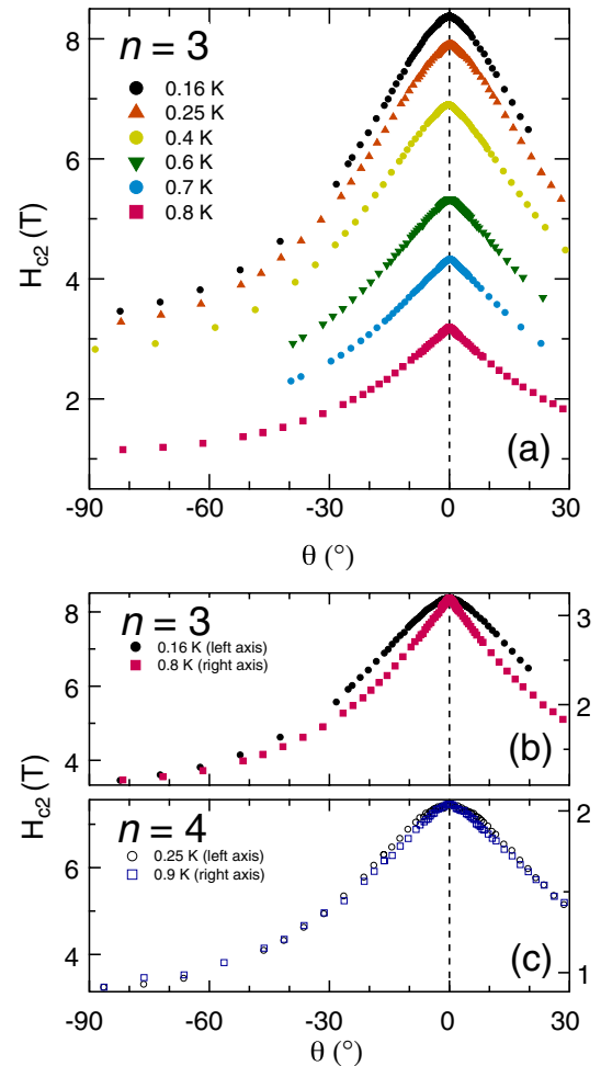
FIG. 2 (color online). (a) Angular dependence of H_{c2} for the n = 3 superlattice. (b) H_{c2}(\theta) of the n = 3 superlattice at 0.16 K and 0.8 K, normalized at H_{c2}(0^\circ) and H_{c2}(90^\circ) , clearly exhibit different curvatures. (c) For reference, H_{c2}(\theta) of the n = 4 superlattice at 0.25 K and 0.9 K, normalized at H_{c2}(0^\circ) and H_{c2}(90^\circ) , are also plotted.
