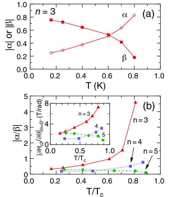
FIG. 4 (color online). (a) The contribution of the linear and quadratic components, characterized by \alpha and \beta , respectively, as a function of temperature for the n = 3 superlattice. (b) The ratio of \alpha/\beta for the n = 3 superlattice as a function of the reduced temperature. The data for n = 4 and n = 5 superlattices are also shown for comparison. Inset: The temperature dependence of |\partial H_{c2}/\partial \theta|_{\theta=0^\circ} extracted experimentally (see text).
