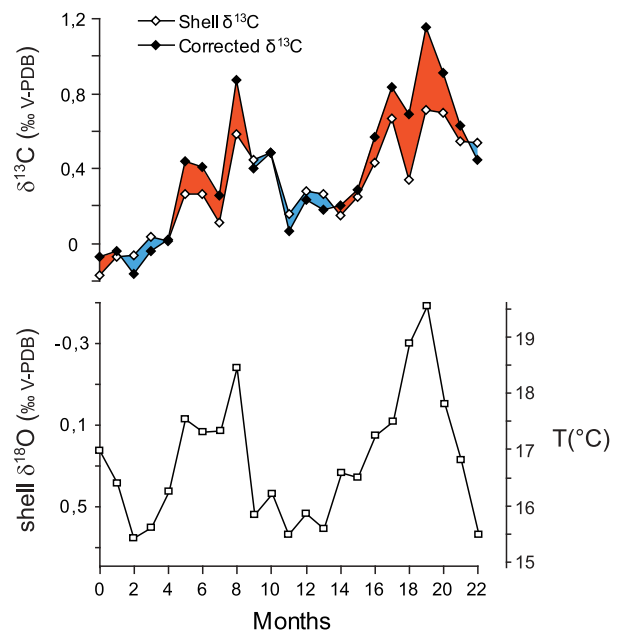
Figure 3. \delta^{13}\text{C} (open diamonds) and \delta^{18}\text{O} (open squares) measured with a monthly resolution along the growth axis of a modern shell (brmd24) collected live in June 2003 on the Llostay beach (close to the QLB site). \delta^{18}\text{O} values were converted to temperature using Carré et al.'s [2005a] equation and a water \delta^{18}\text{O} value of 0.18‰(V-SMOW). \delta^{13}\text{C}_{\text{corr}} values (closed diamonds) were calculated from shell \delta^{13}\text{C} corrected from the temperature fractionation effect and the Suess effect. Positive corrections appear in red and negative corrections in blue.
